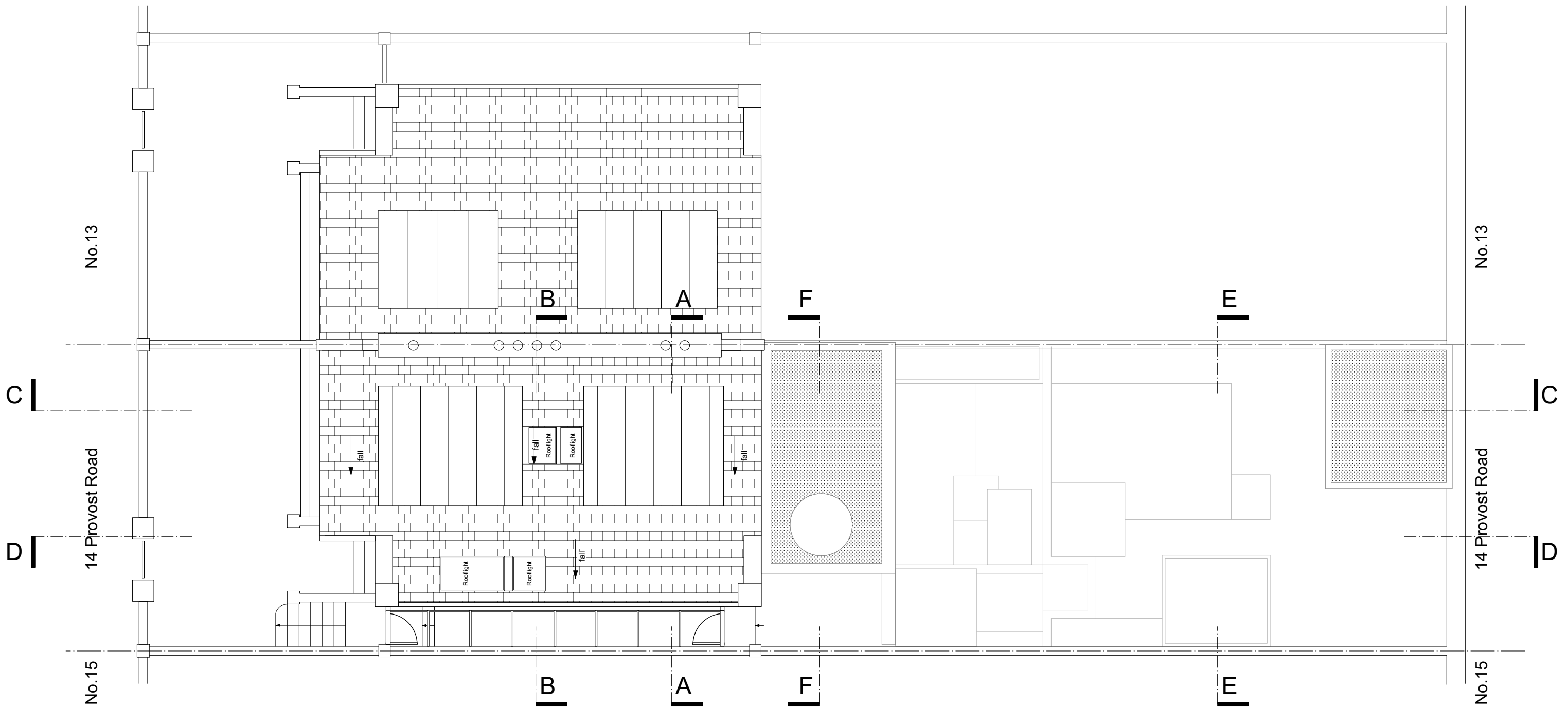
Roof Plan PLAN
