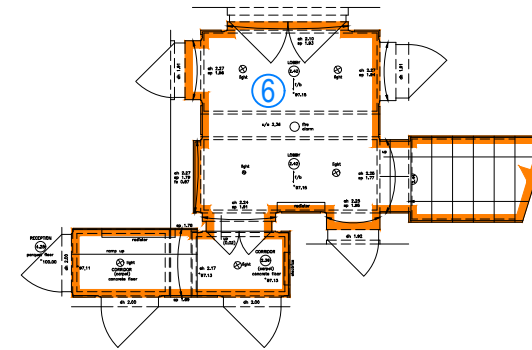
EXISTING LOWER GROUND FLOOR PLAN Scale 1:100
