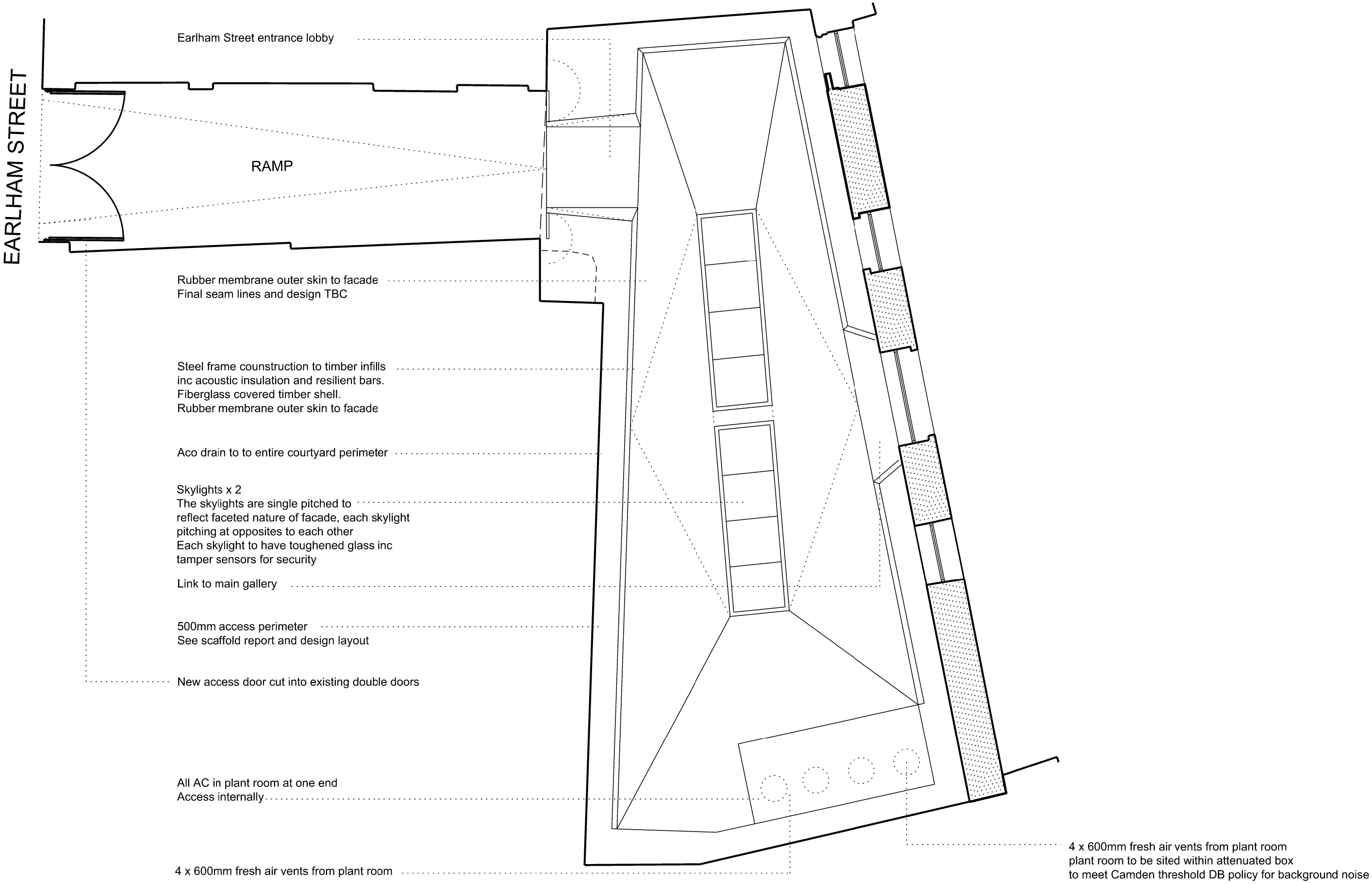
PHASE 2 SHELTON STREET PROPOSED ROOF PLAN
