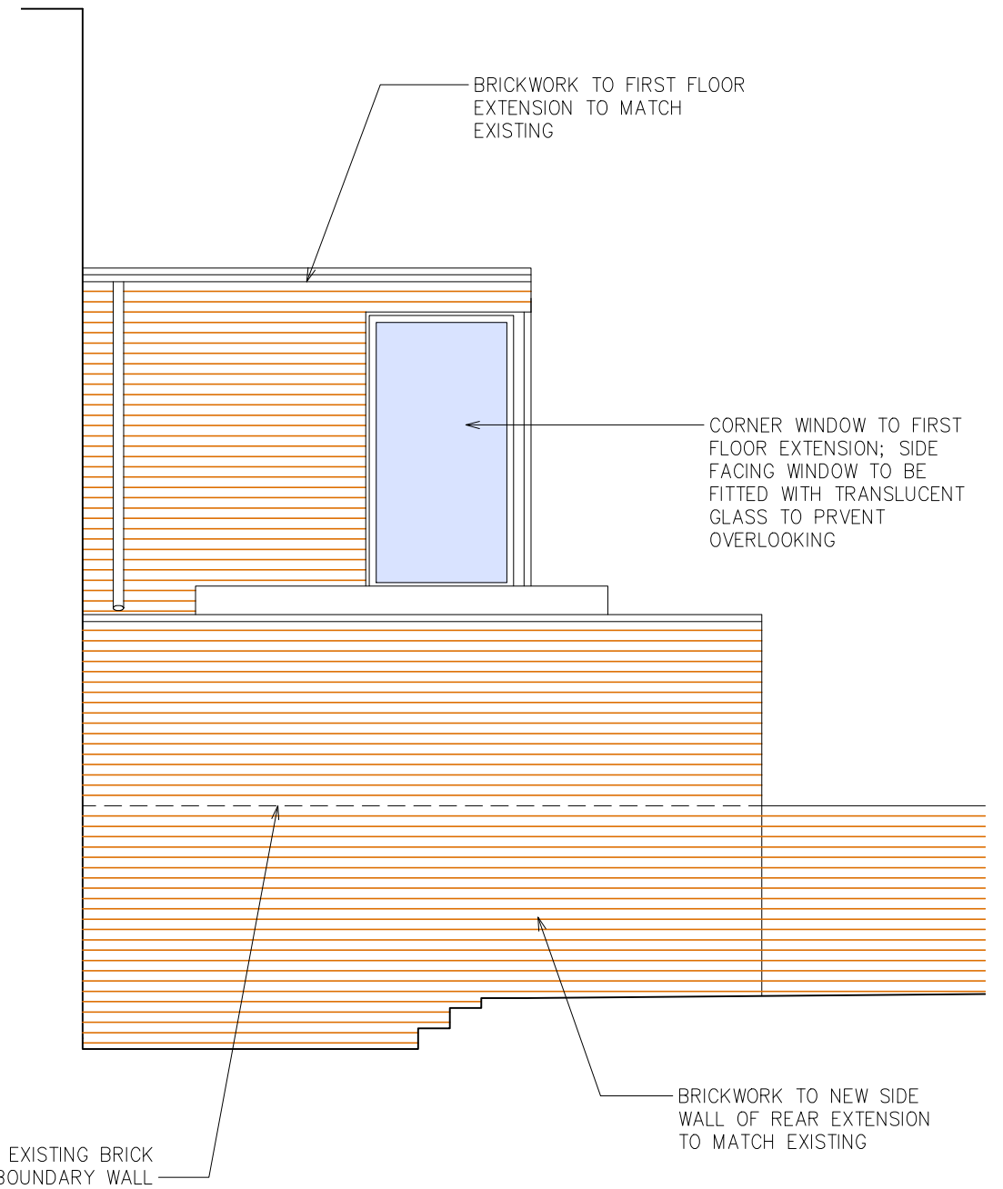
2 PROPOSED SIDE ELEVATION 1 : 50
