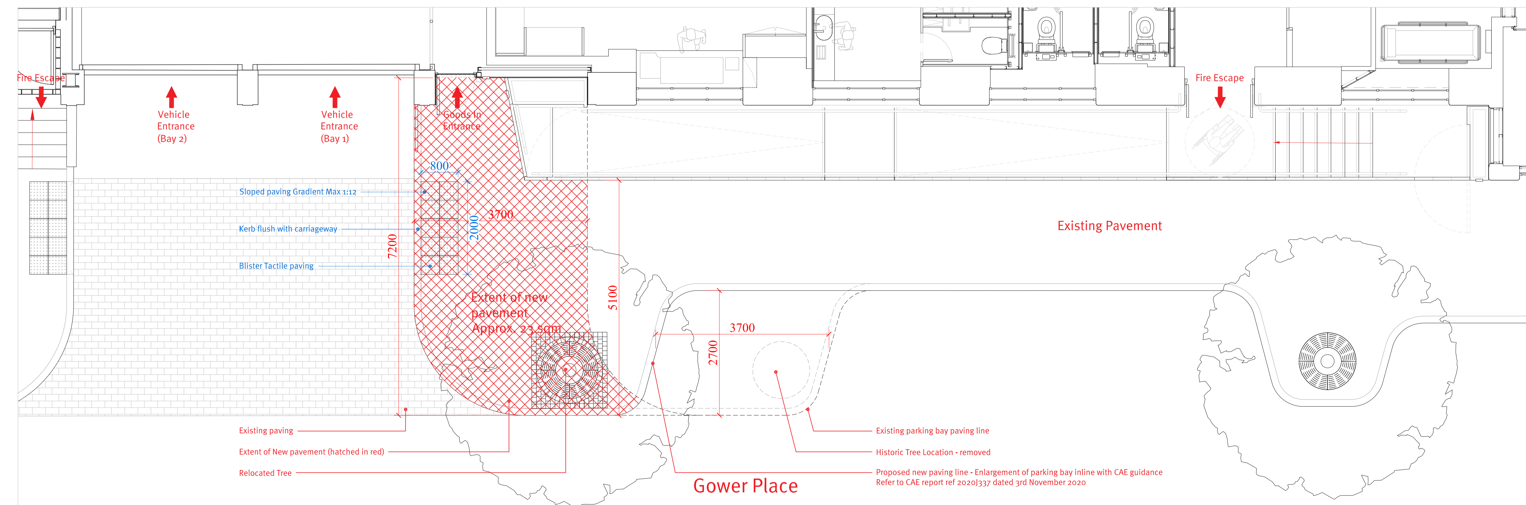
02 Proposed Detail Plan 1:50 @ A1
