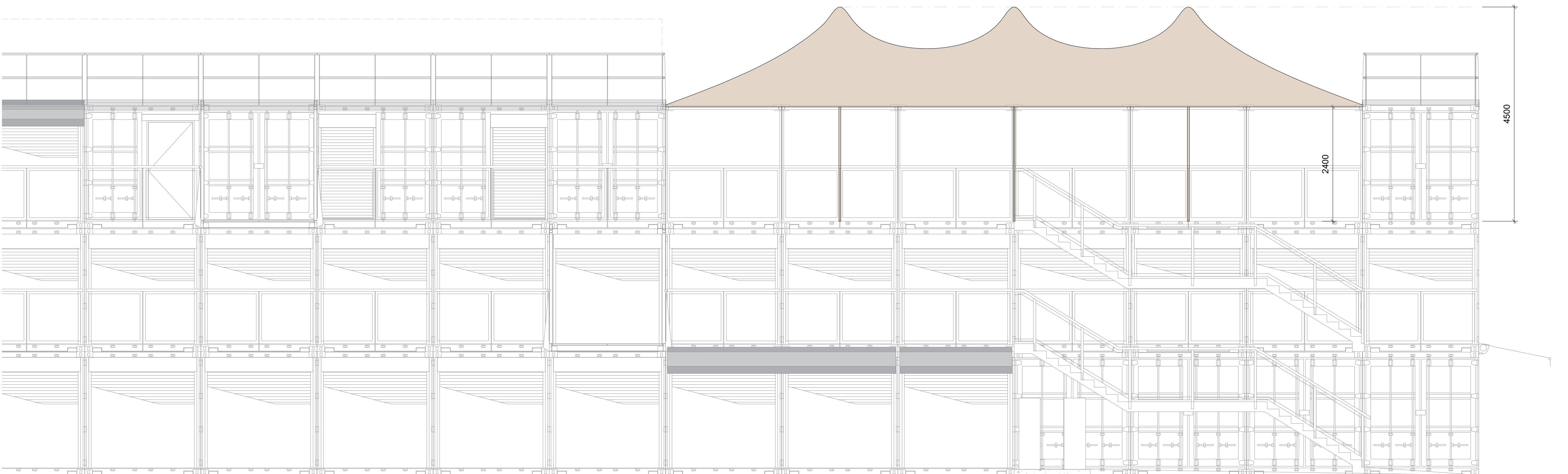
02 ELEVATION B-B SCALE 1:50 @ A1
