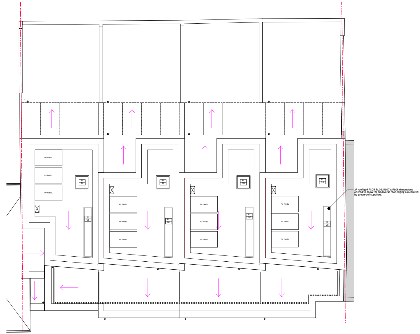
01 PROPOSED ROOF PLAN
