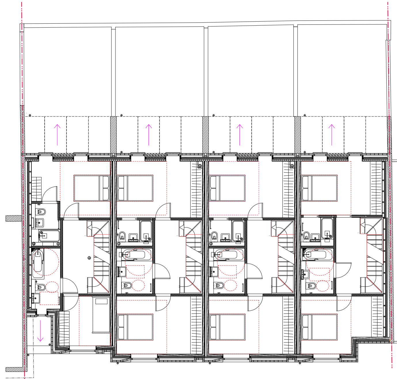
01 PROPOSED FIRST FLOOR PLAN
