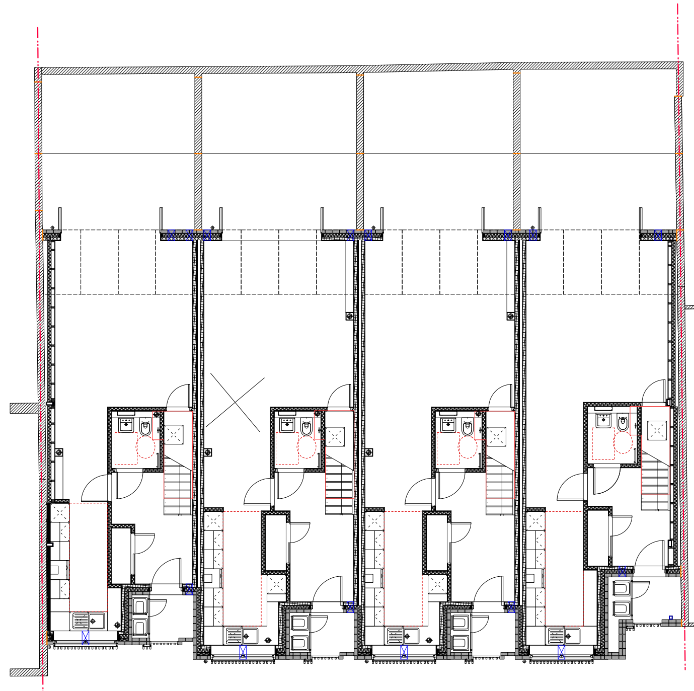
01 PROPOSED GROUND FLOOR PLAN
