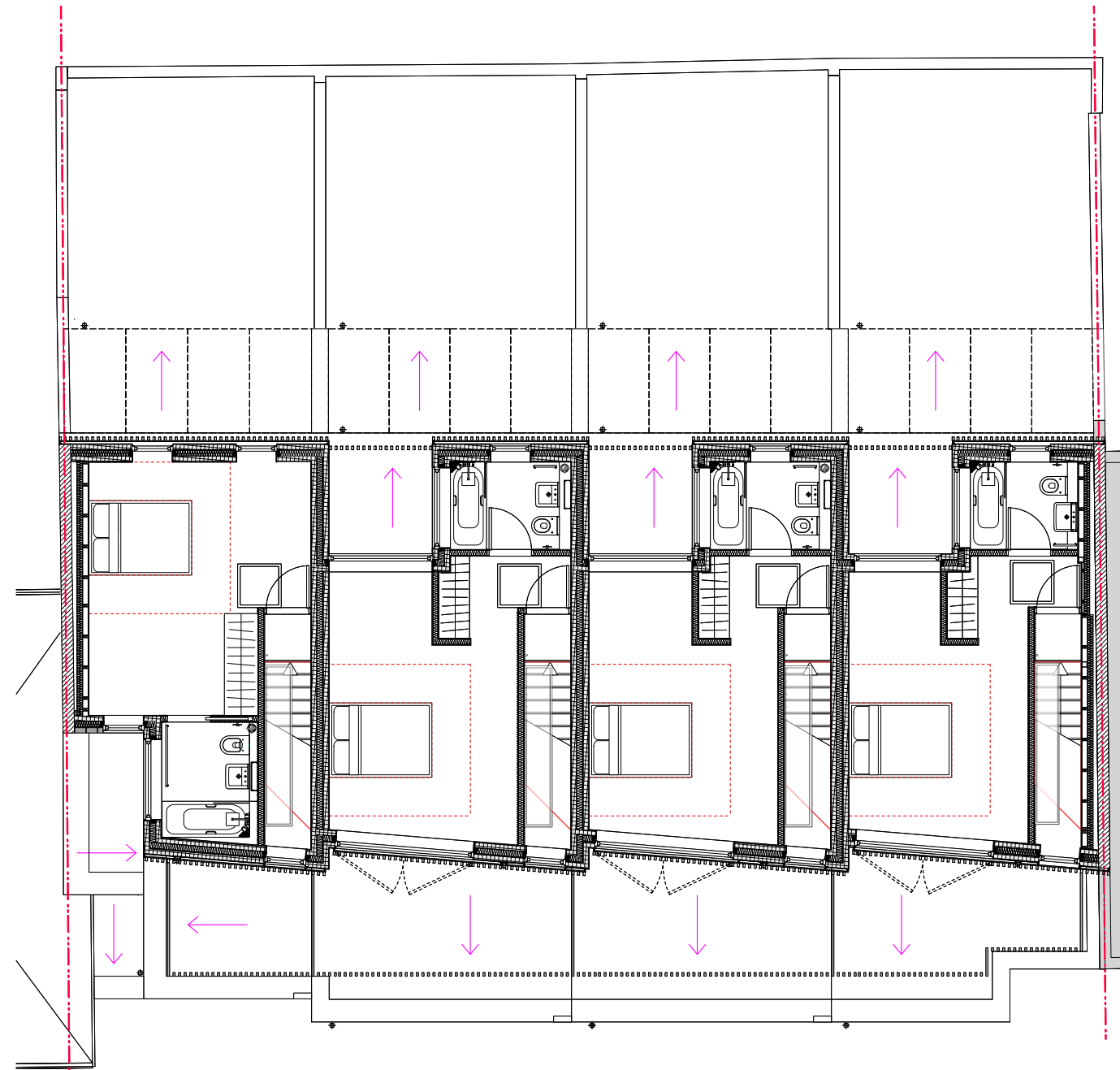
01 PROPOSED SECOND FLOOR PLAN
