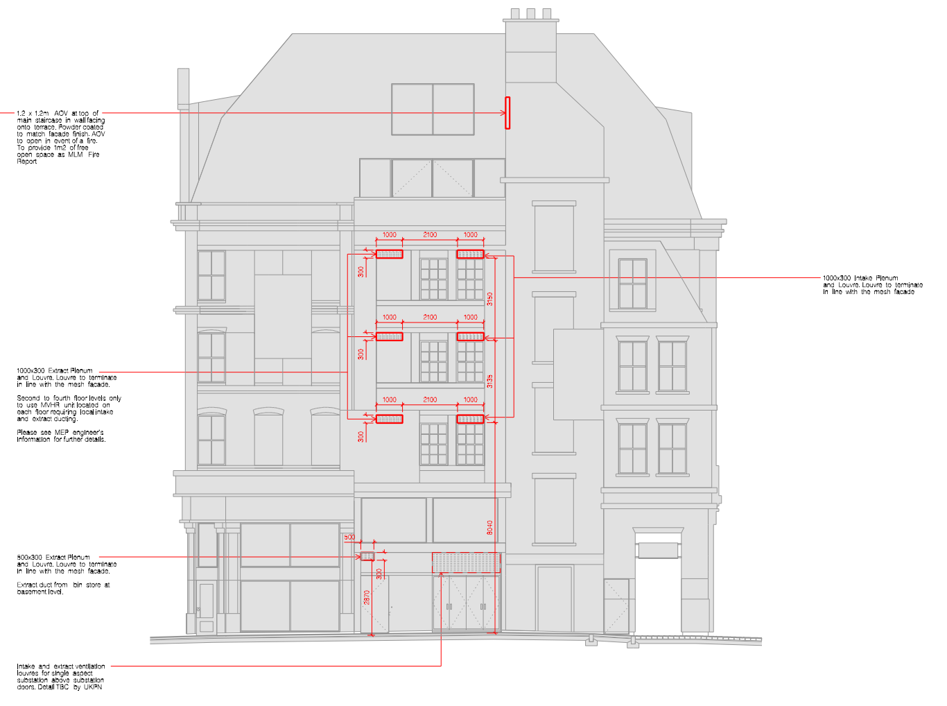
② WEST ELEVATION VENTILATION LOUVRE LOCATION
