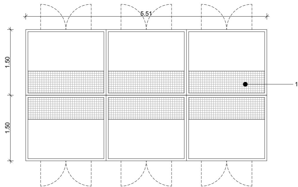
ROOF PLAN
