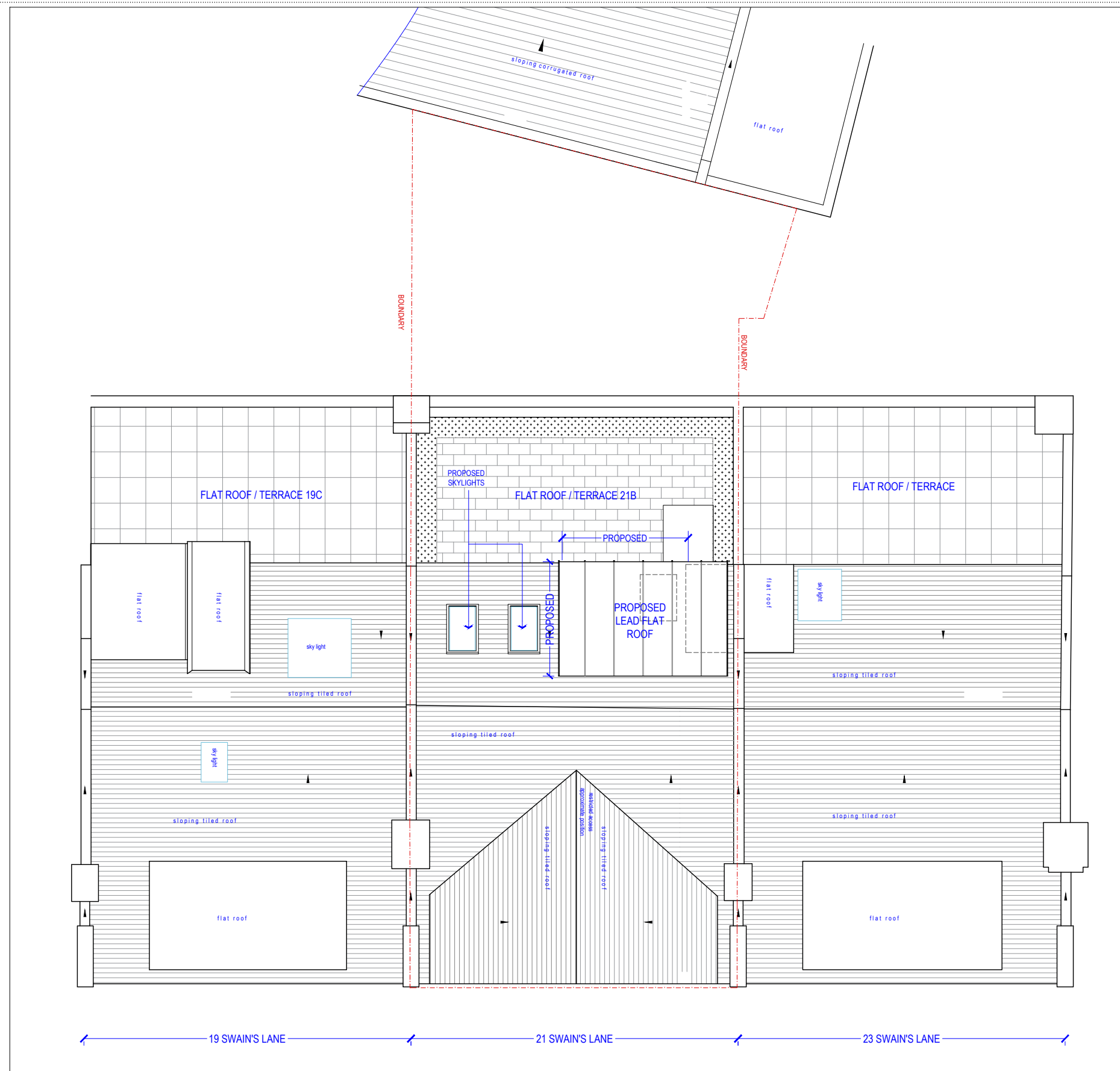
[01] PROPOSED ROOF PLAN
