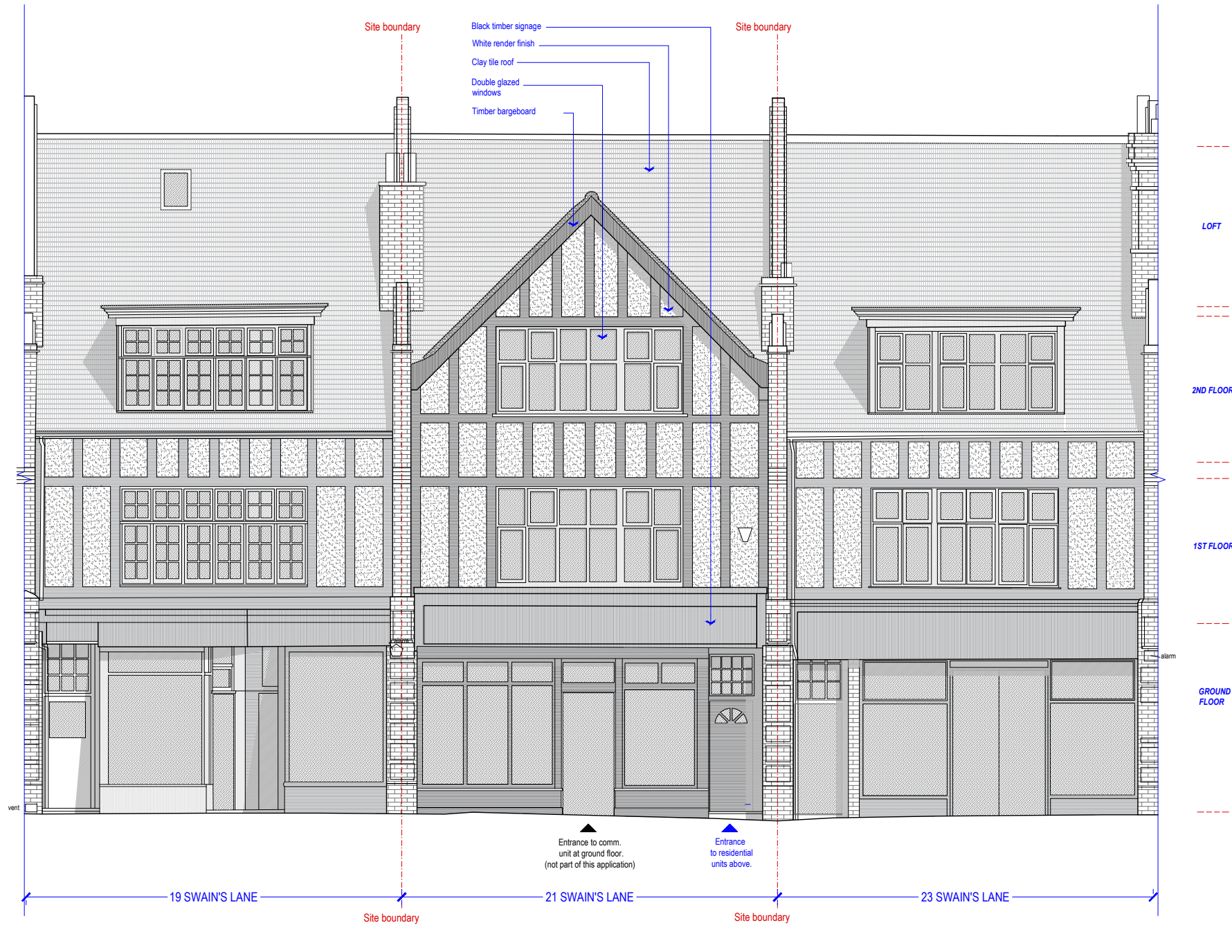
[01] EXISTING FRONT ELEVATION
