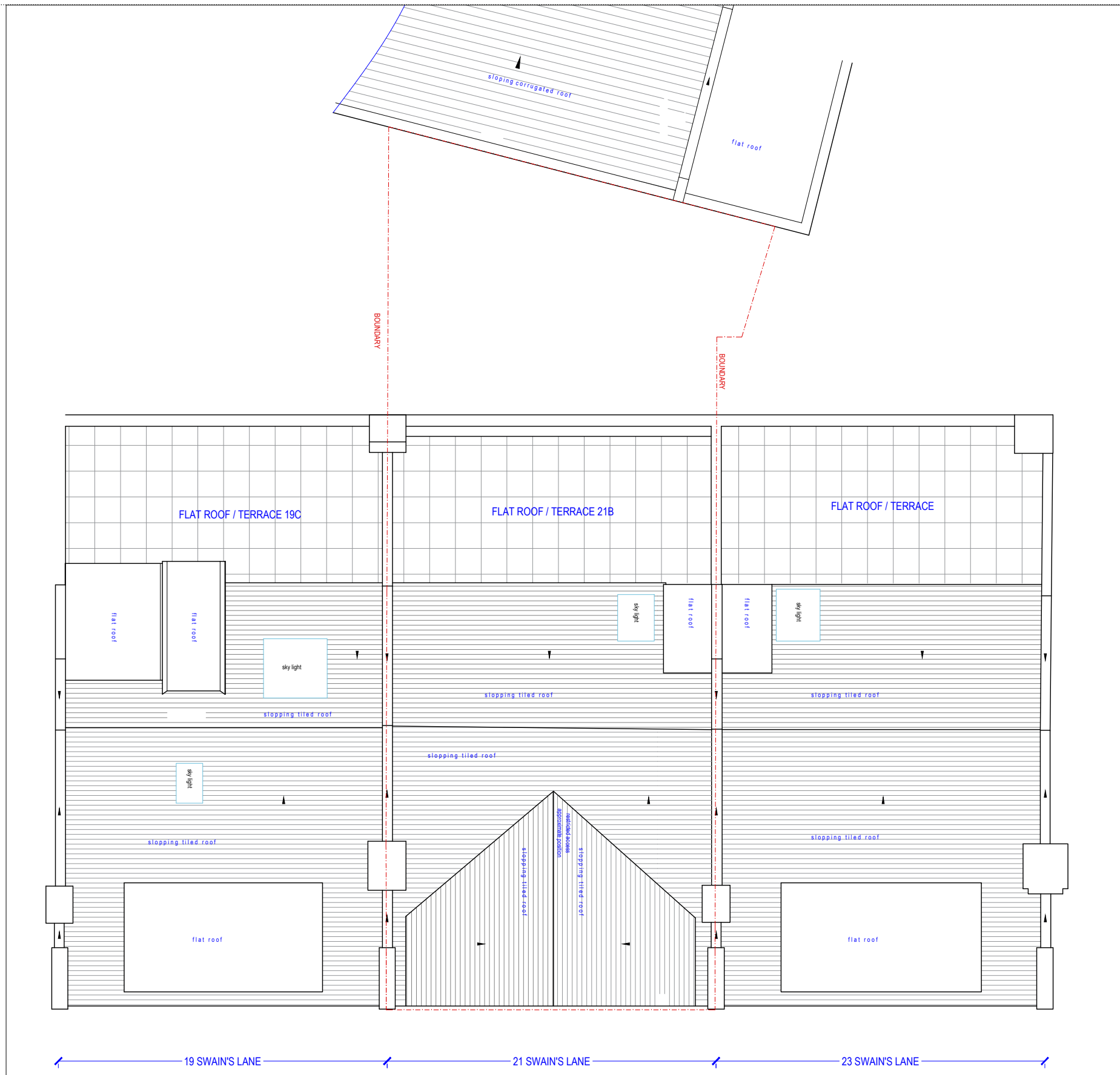
[01] EXISTING ROOF PLAN
