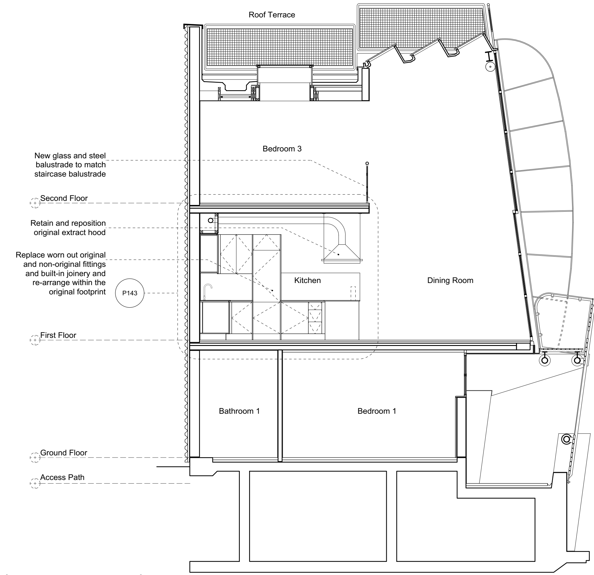
Proposed_Section A-A
