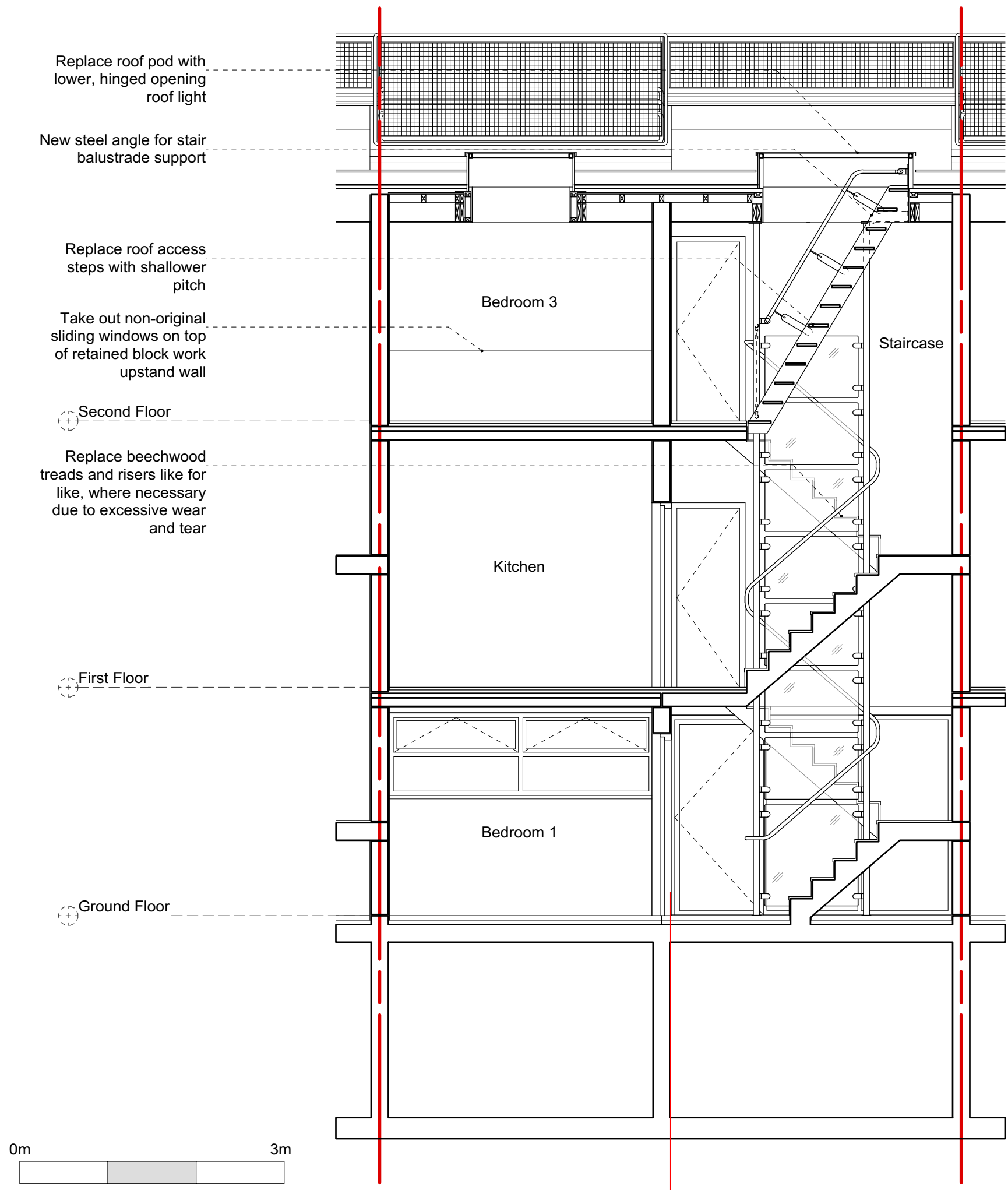
Proposed_Section C-C
