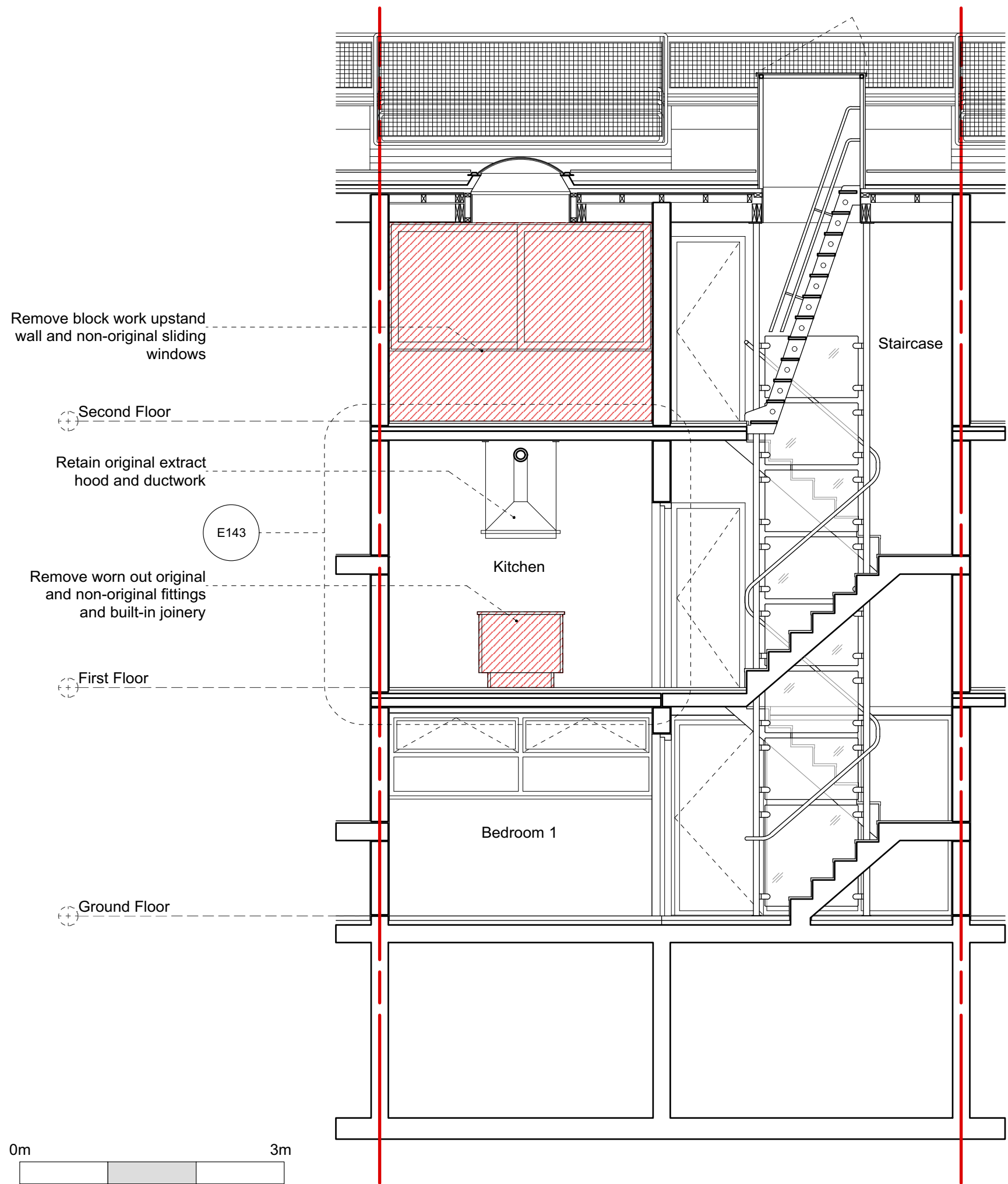
As Existing_Section C-C
