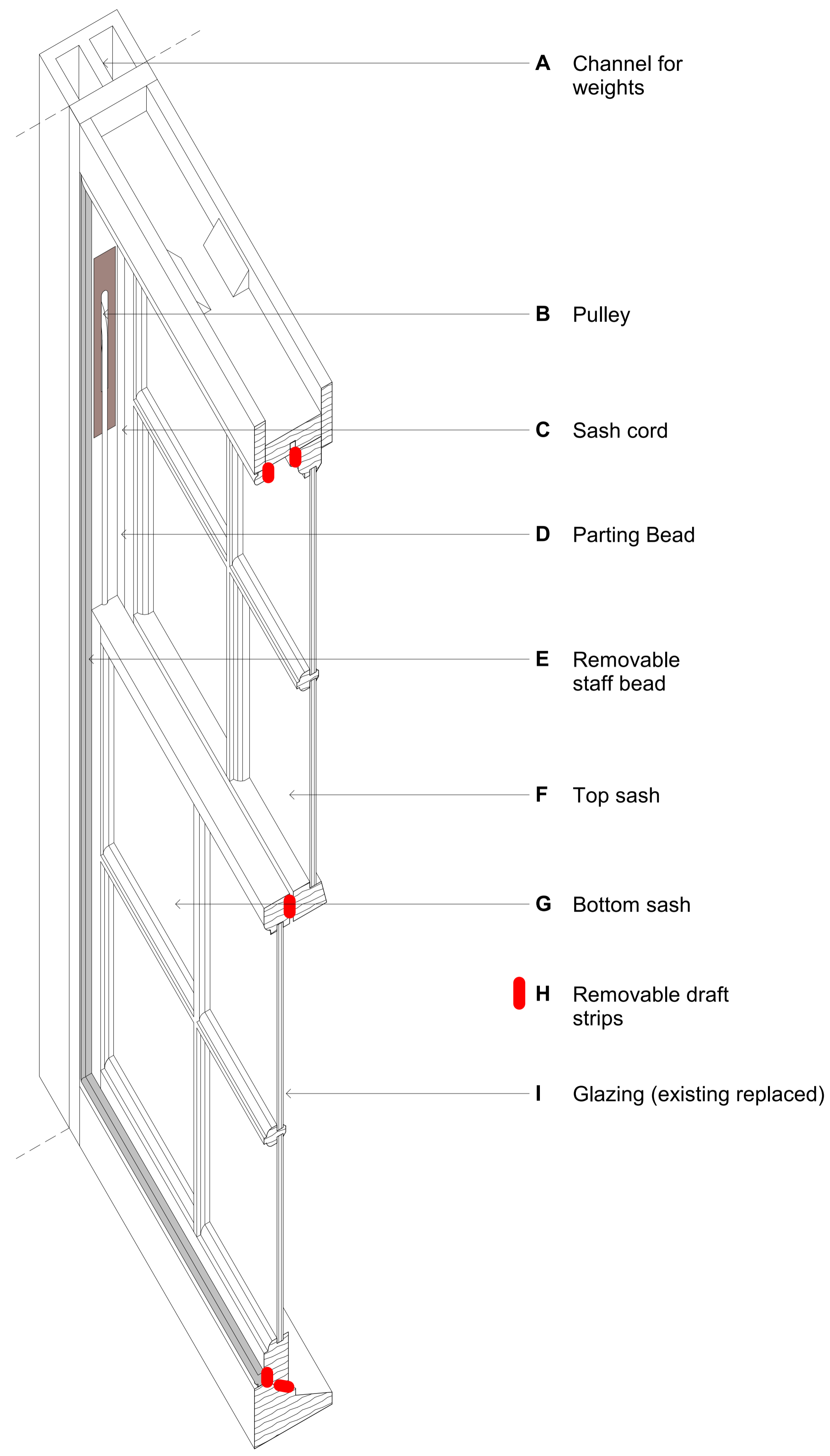
Proposed Window Overhaul Schematic Scale 1 : 5
