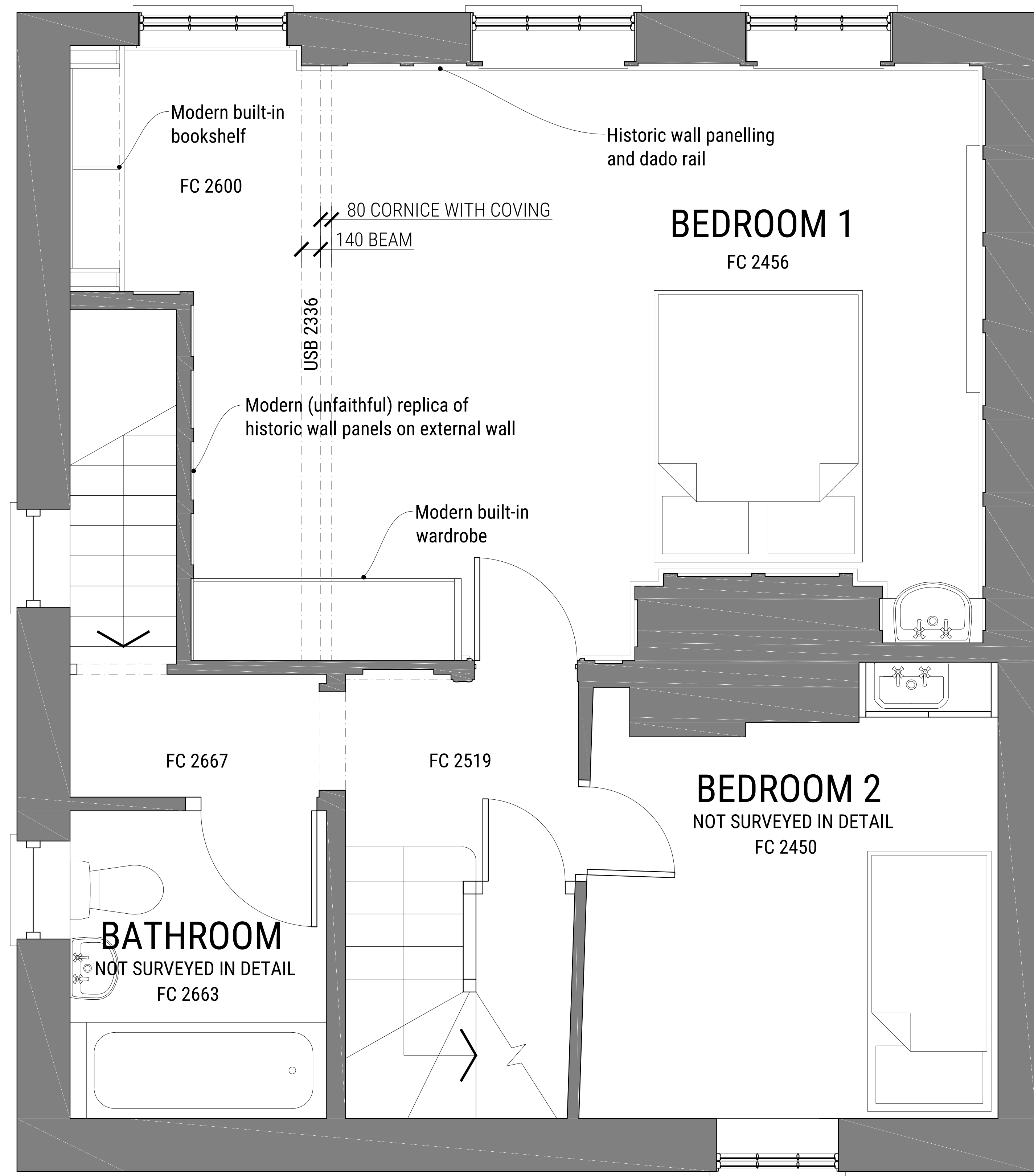
01 Existing First Floor Plan Scale 1:20@A1
