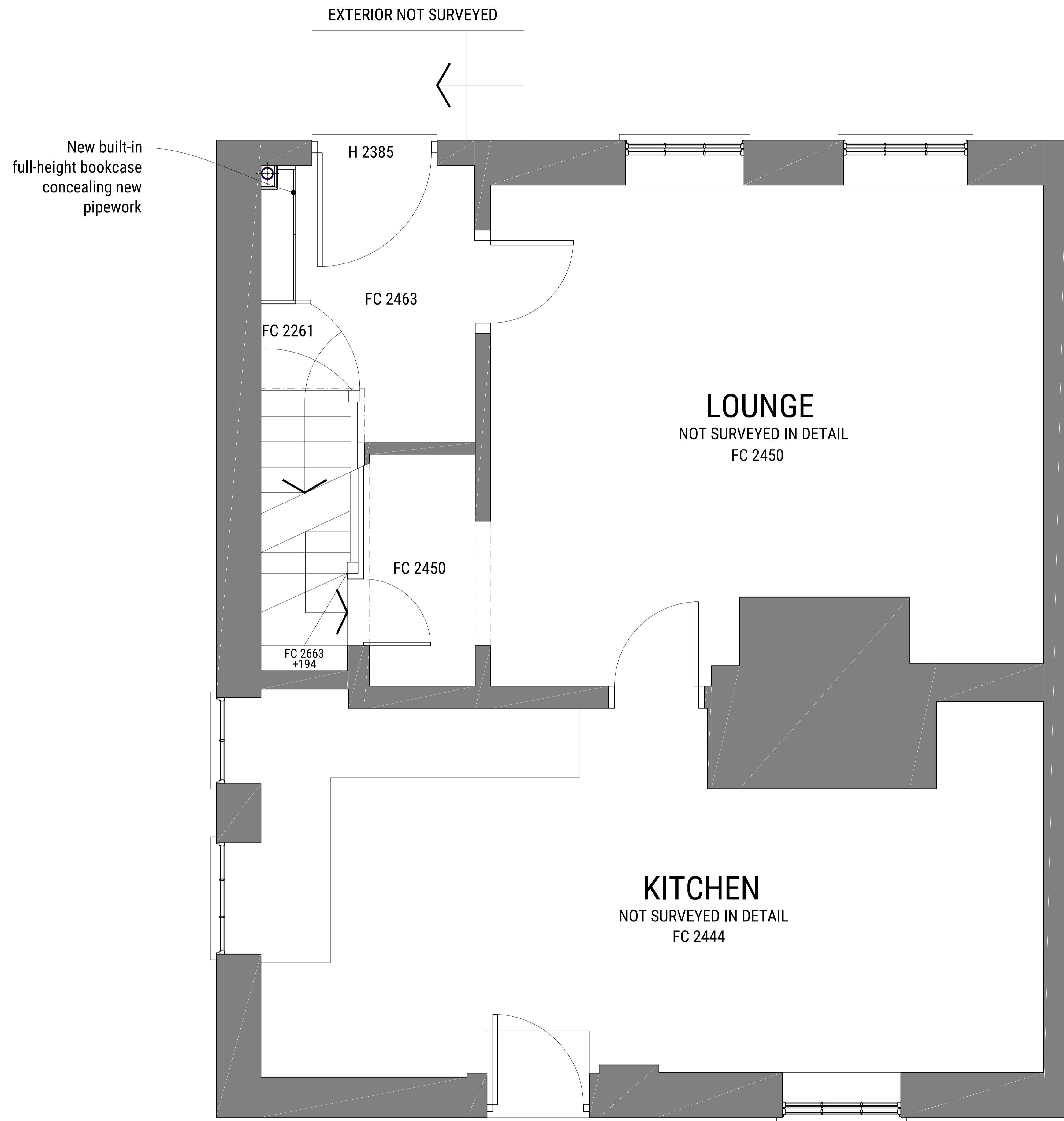
01 Proposed Ground Floor Plan Scale 1:20@A1
