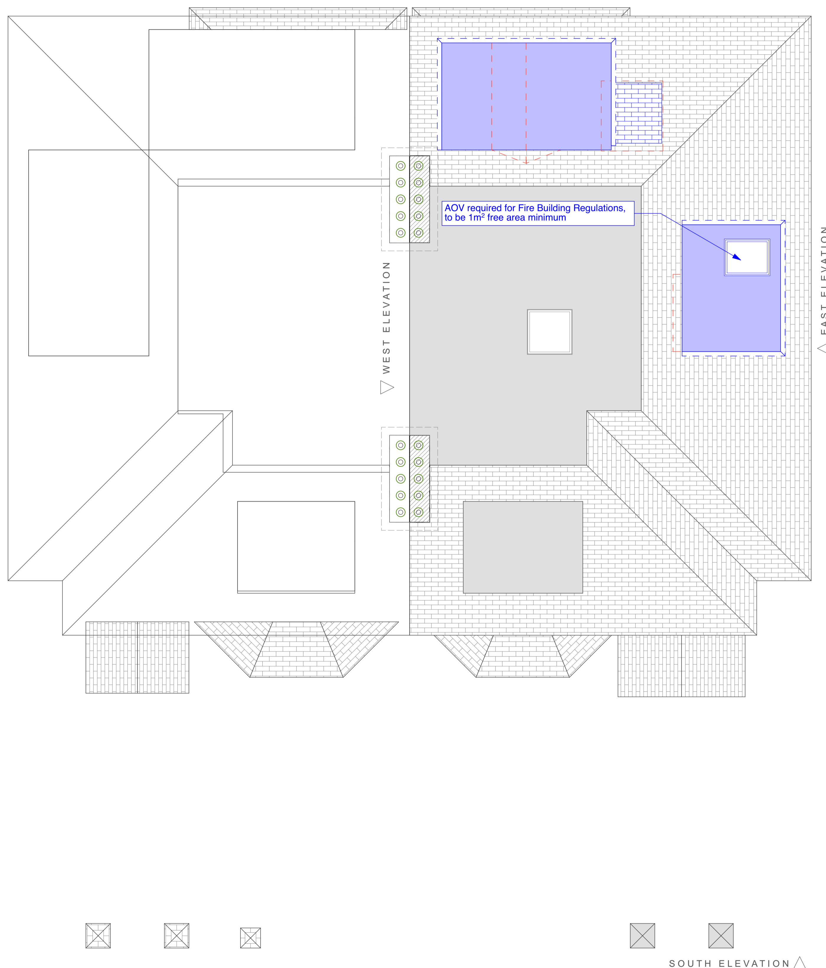
PROPOSED ROOF 1:50
