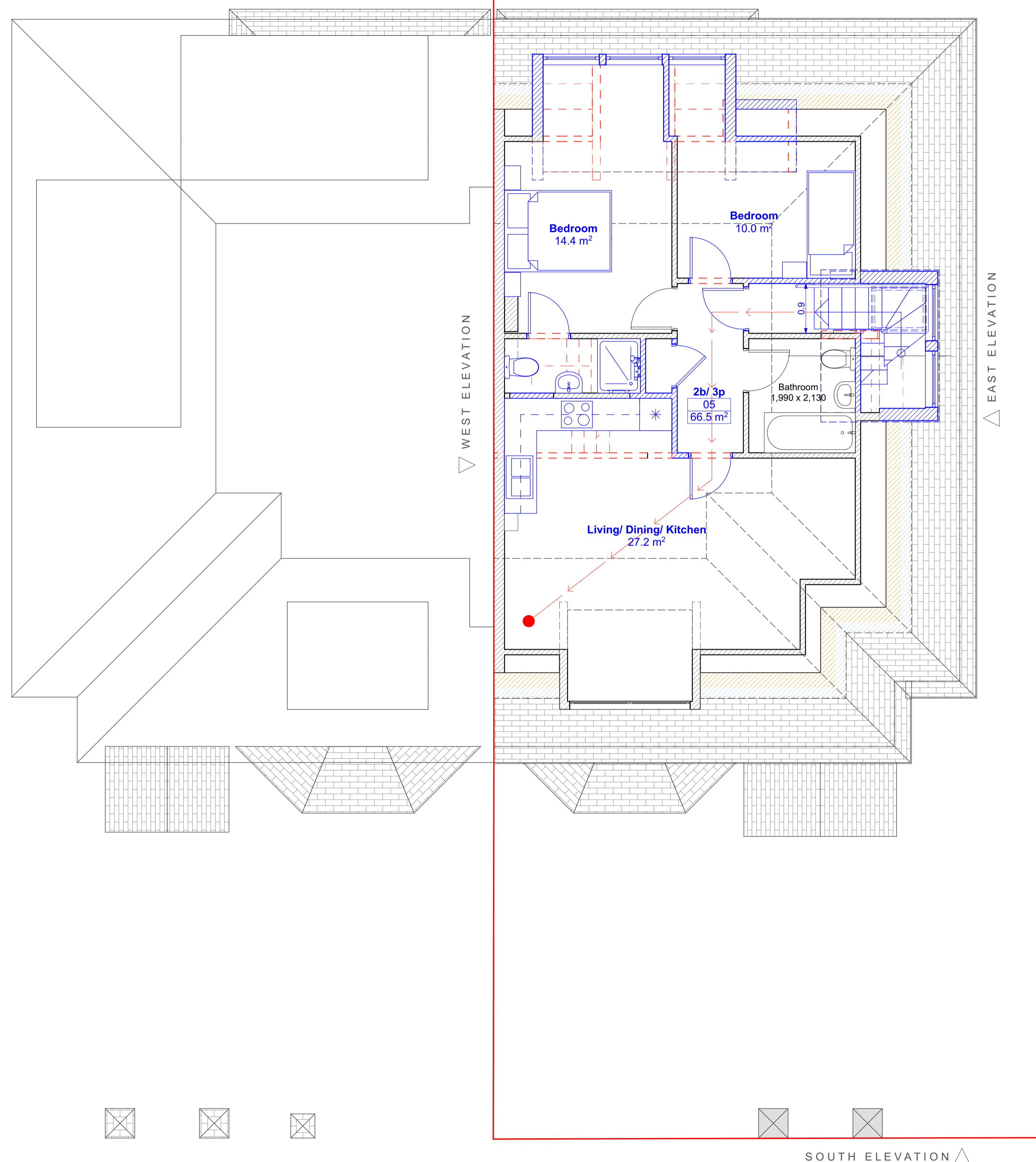
PROPOSED ATTIC 1:50
