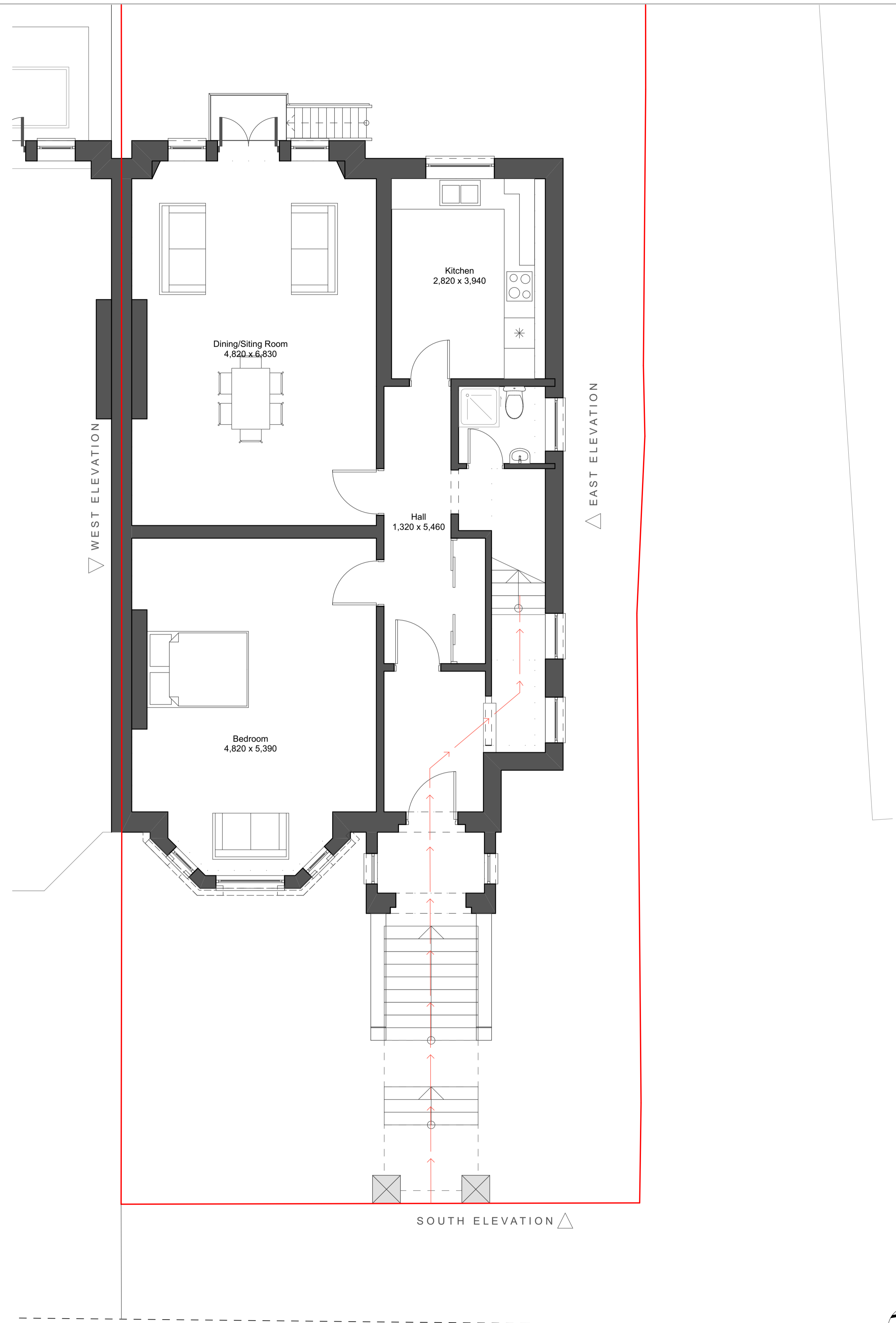
EXISTING GROUND 1:50
