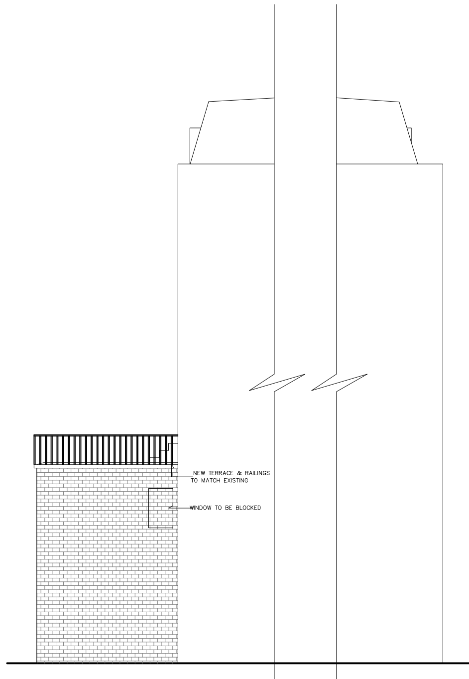
PROPOSED FLANK ELEVATION
