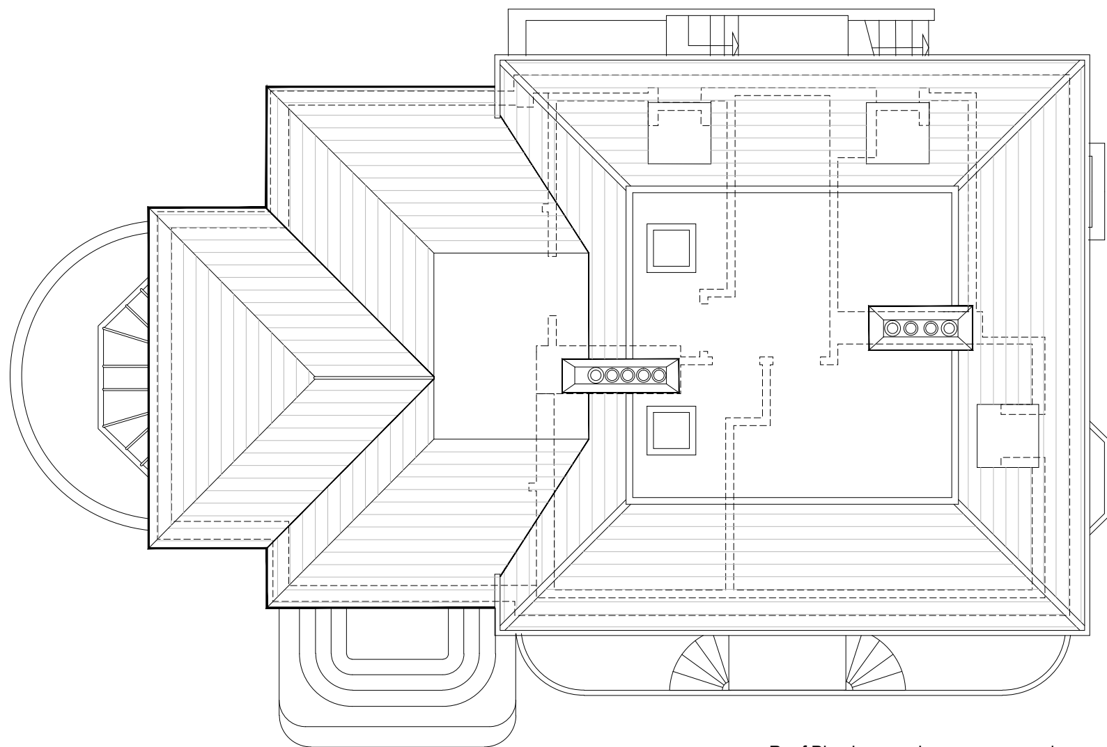
Roof Plan has no changes proposed
