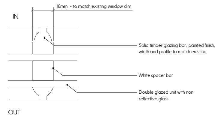
Section through glazing bar, scale 1:1
