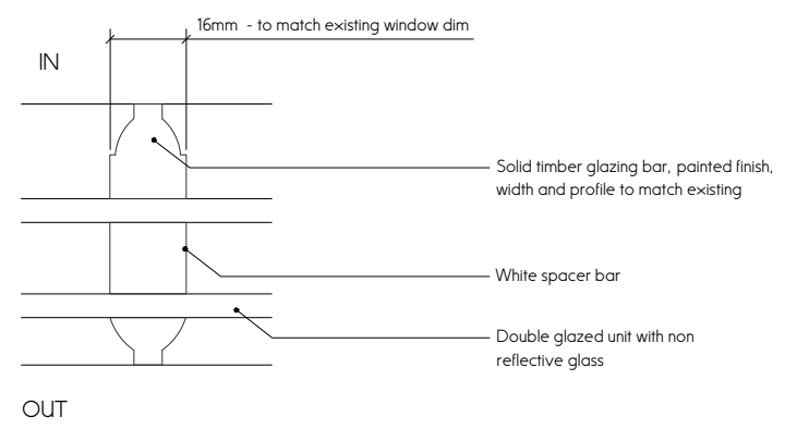
Section through glazing bar, scale 1:1
