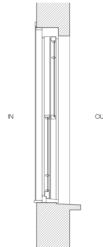
Section AA
