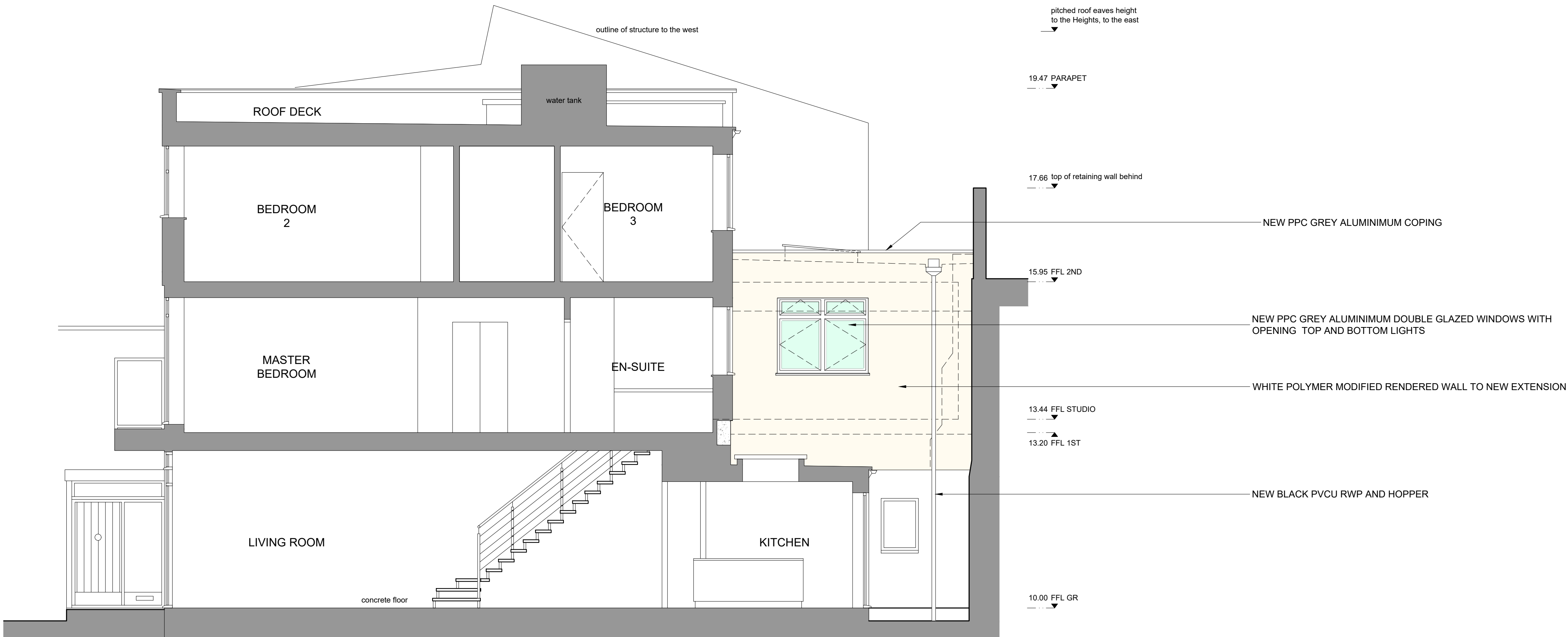
1 PROPOSED SECTION AA A1 @ Scale: 1:50
