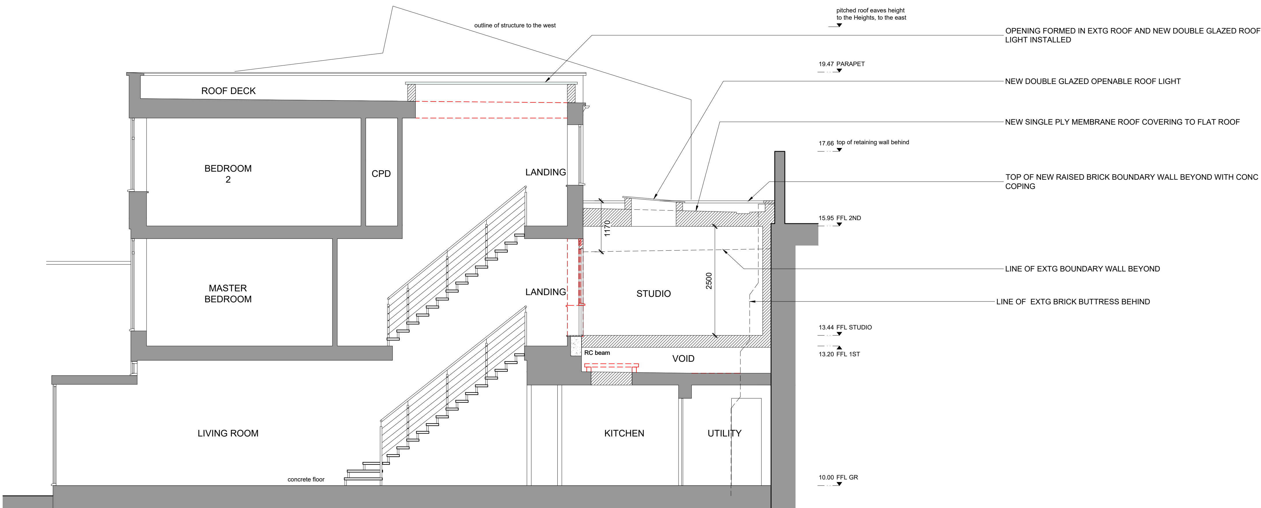
2 PROPOSED SECTION BB A1 @ Scale: 1:50
