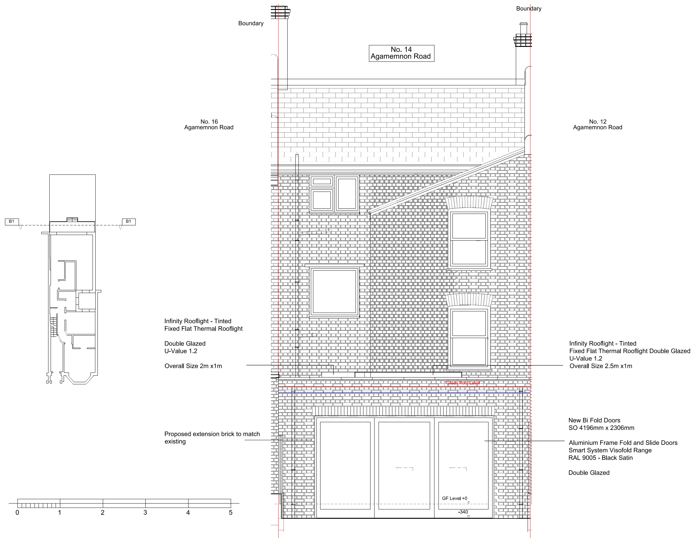
Rear Elevation B-B
