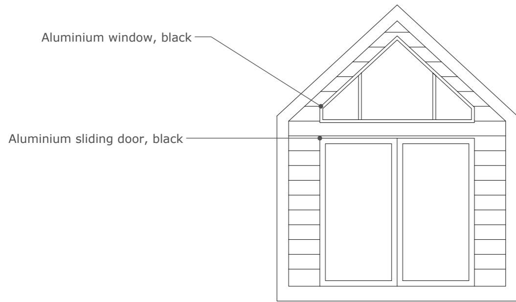
North Elevation
