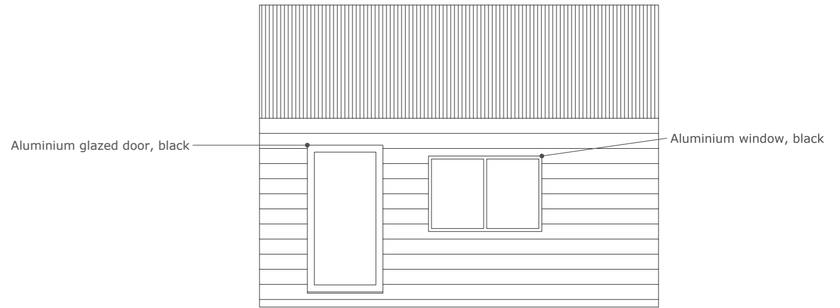
East Elevation
