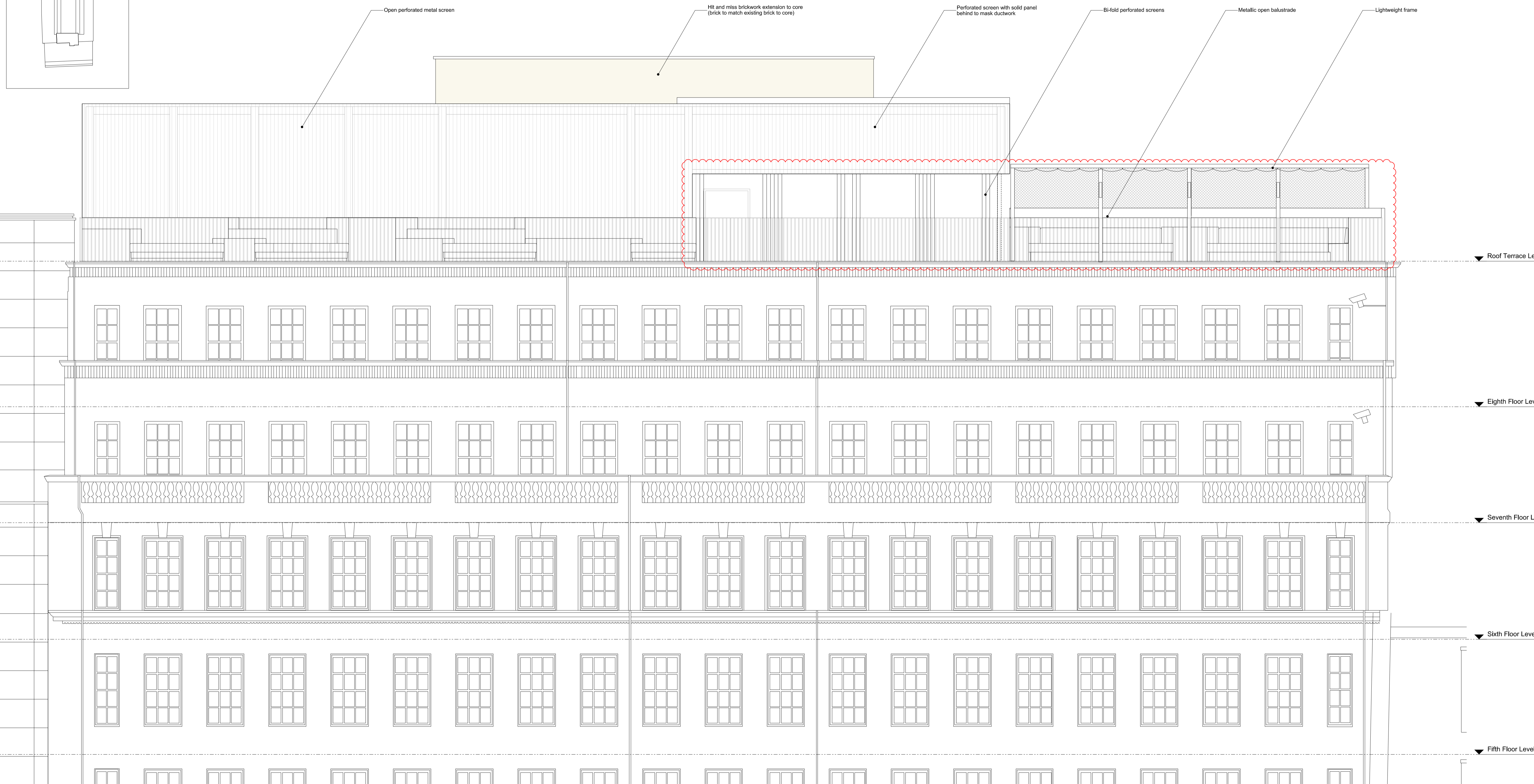
01 Proposed South Elevation 1:50
