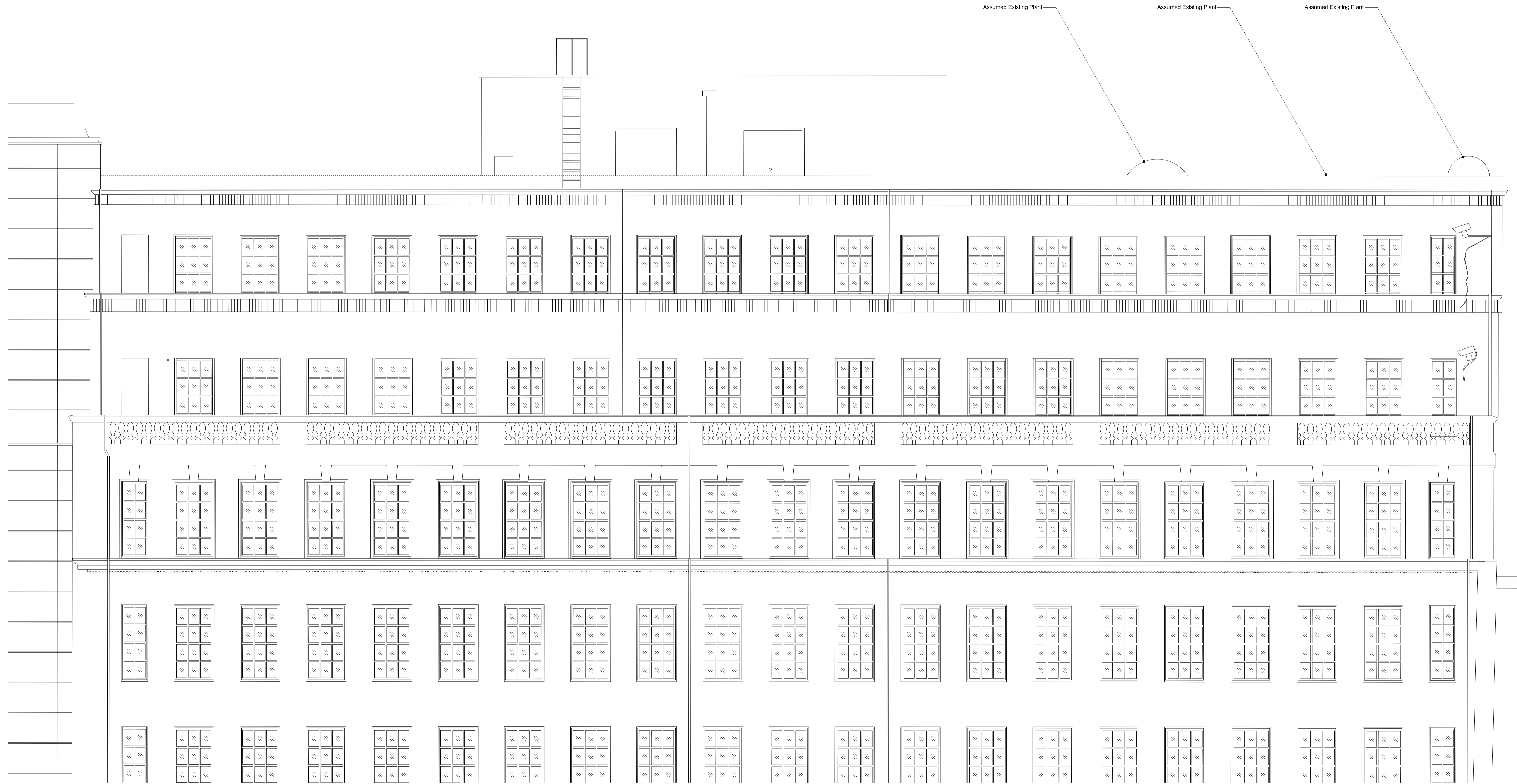
01 Existing South Elevation 1:50
