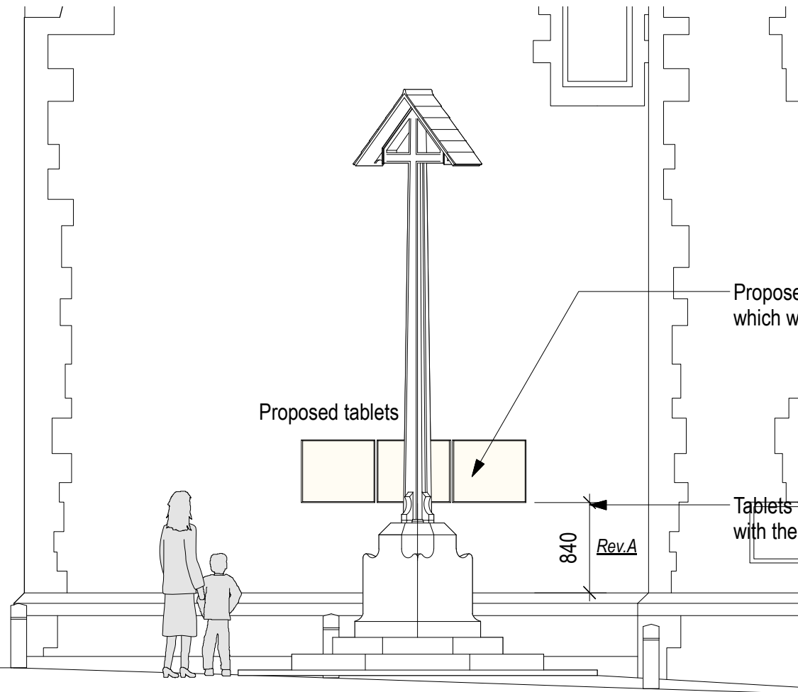
West Elevation 1:50
