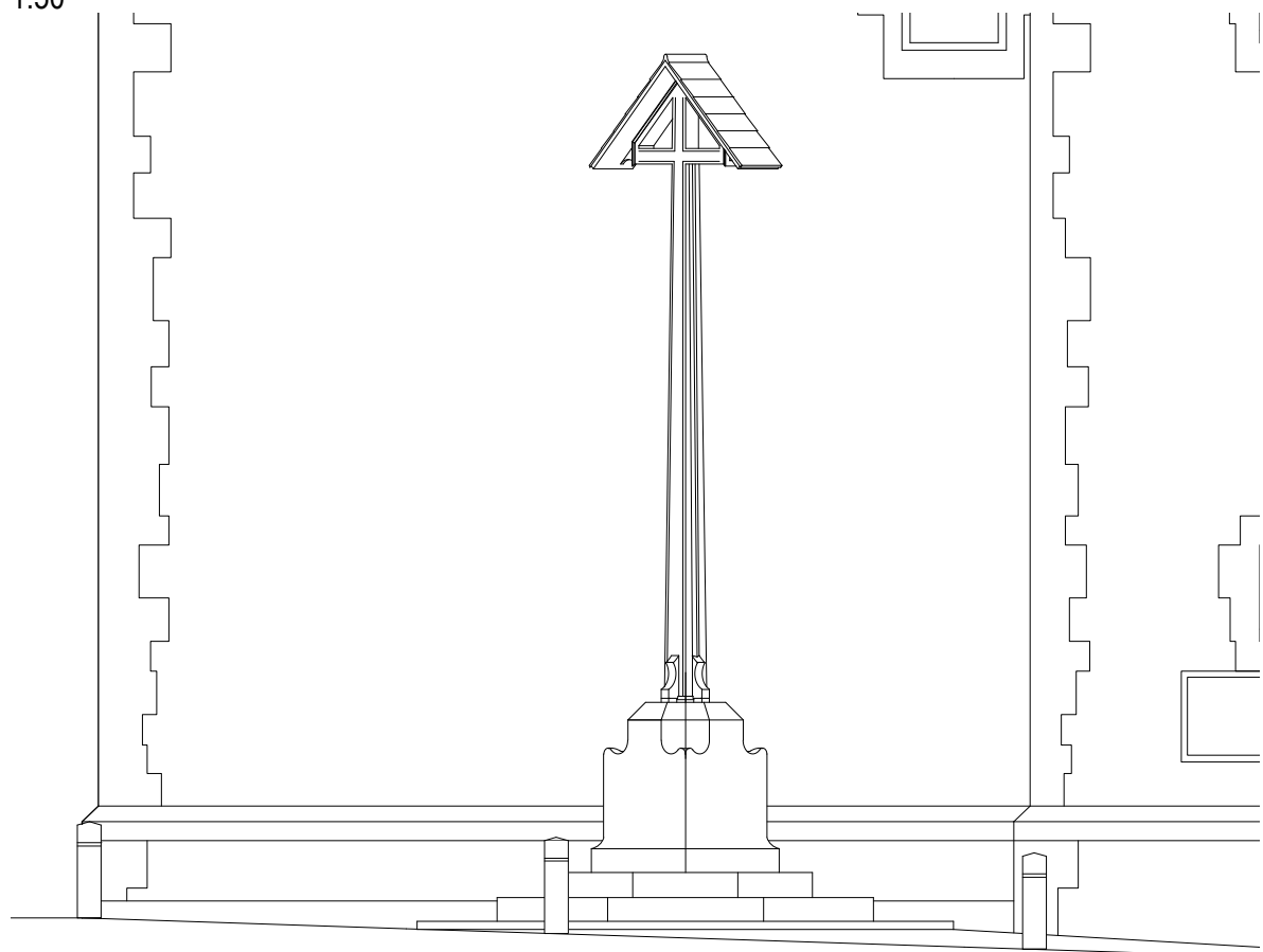
West Elevation 1:50
