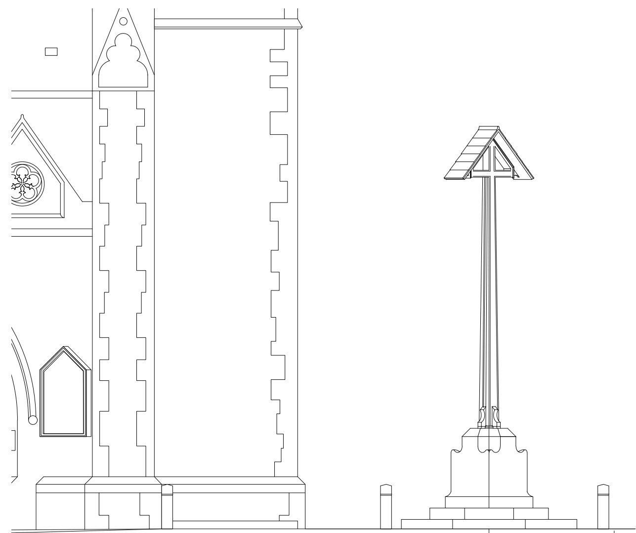
North Elevation 1:50
