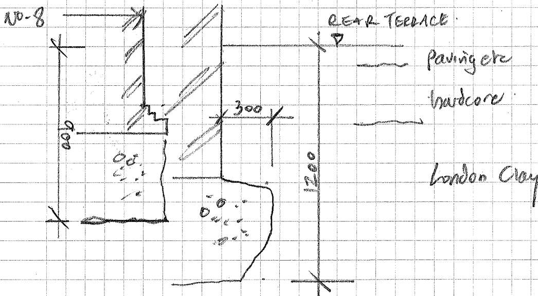
NORTH COLUMN 1:20 (looking north)
