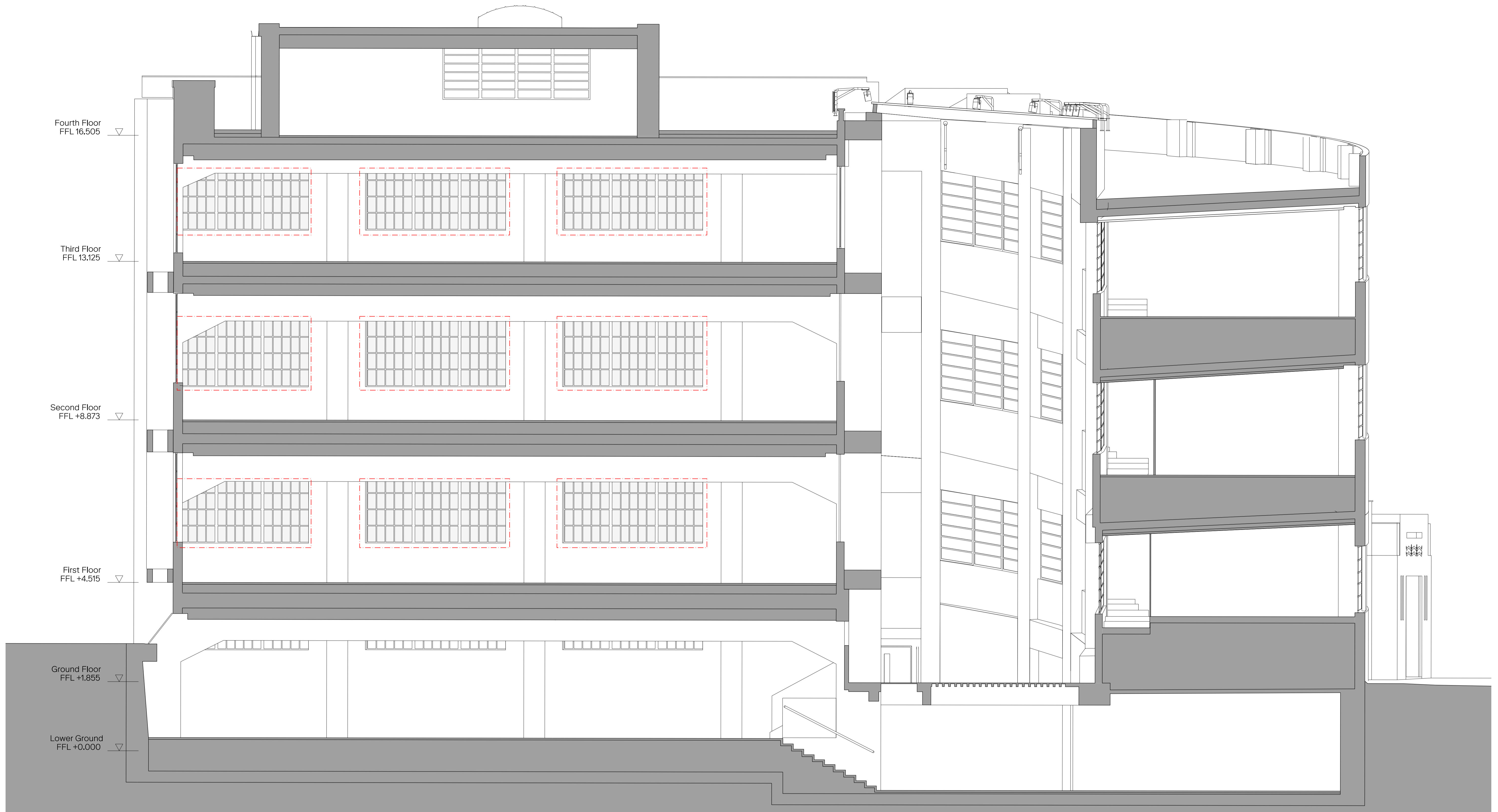
01 Typical cross section 1:50@A1
