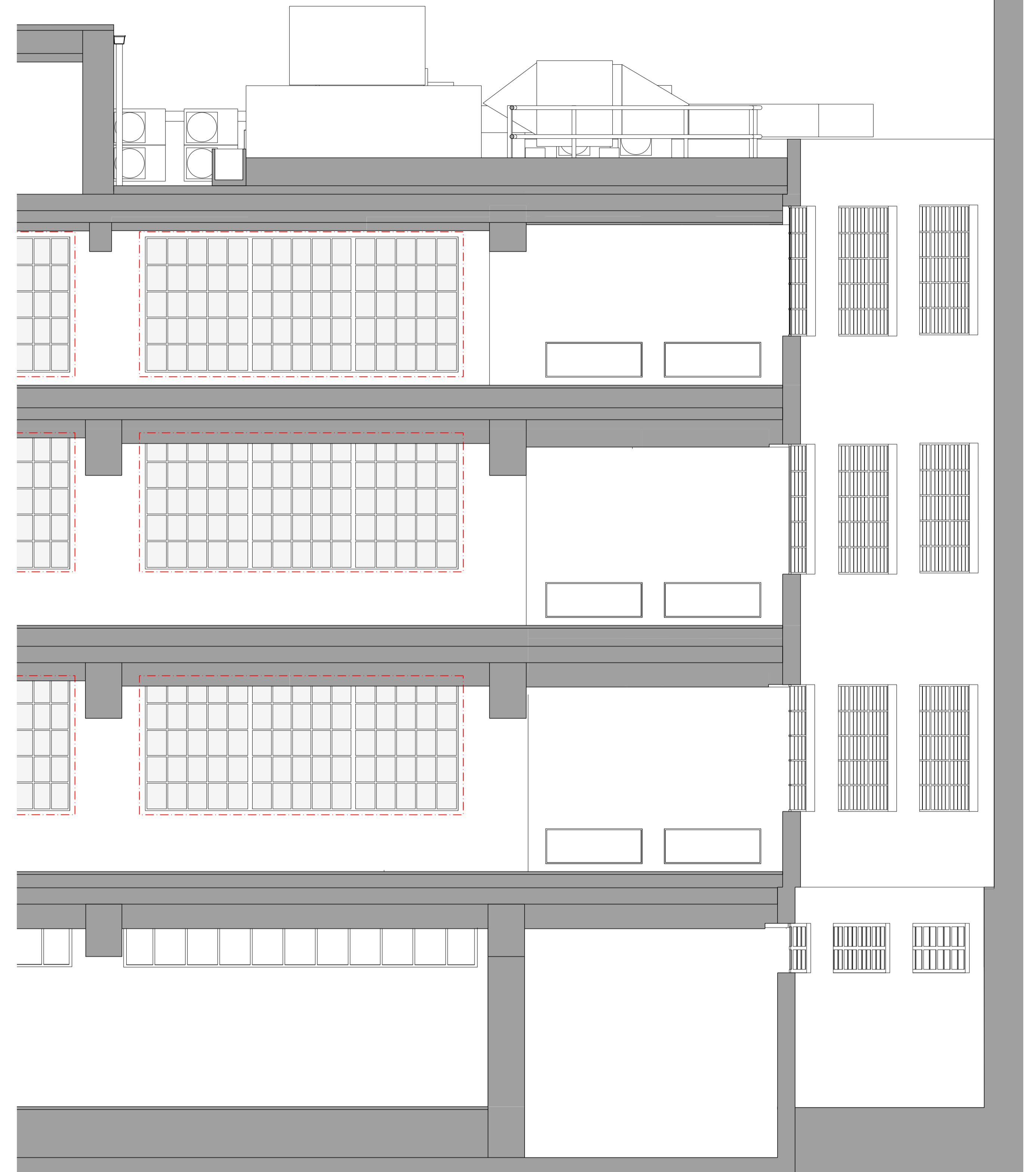
02 Typical long section 1:50@A1
