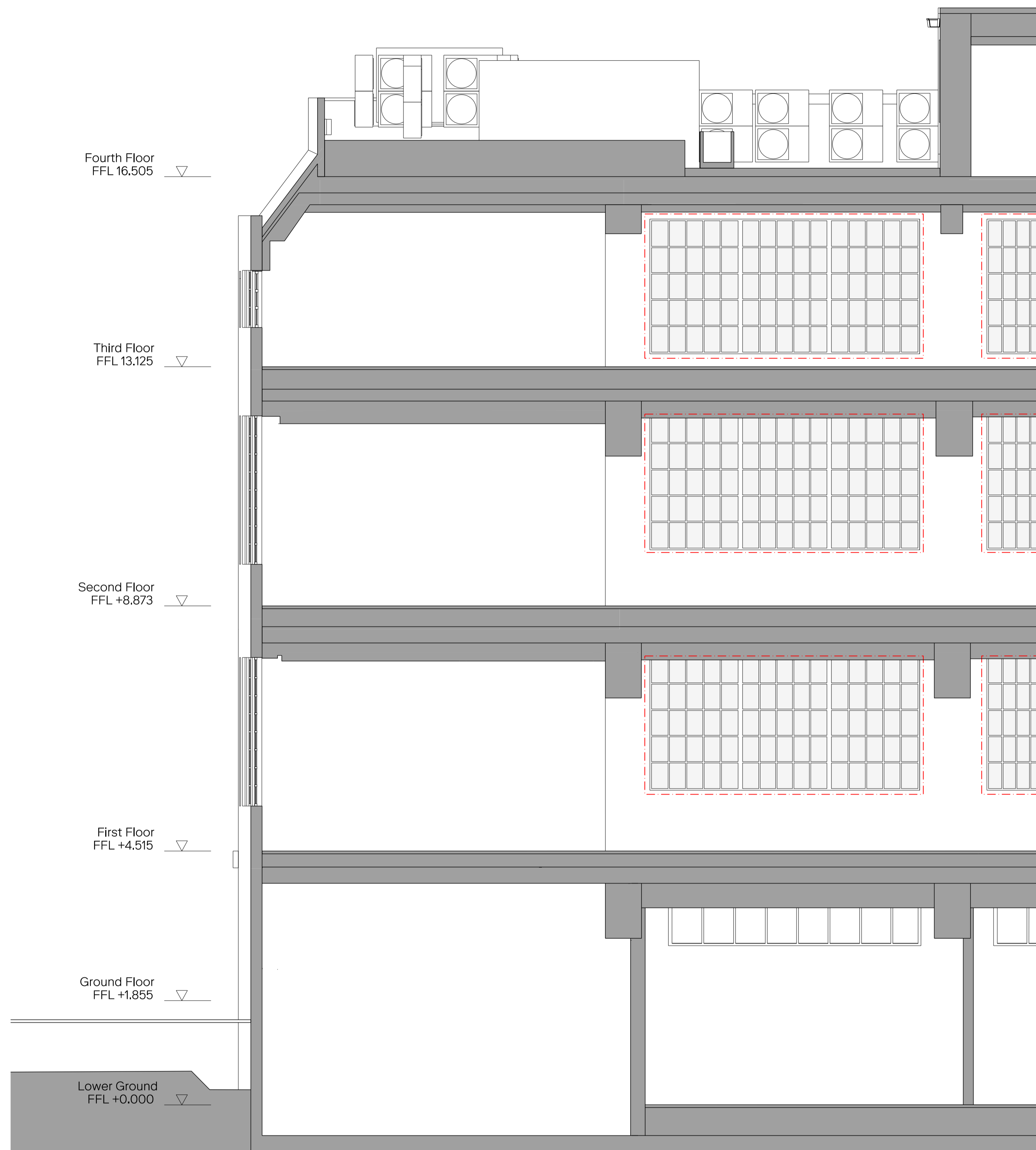
01 Typical long section 1:50@A1
