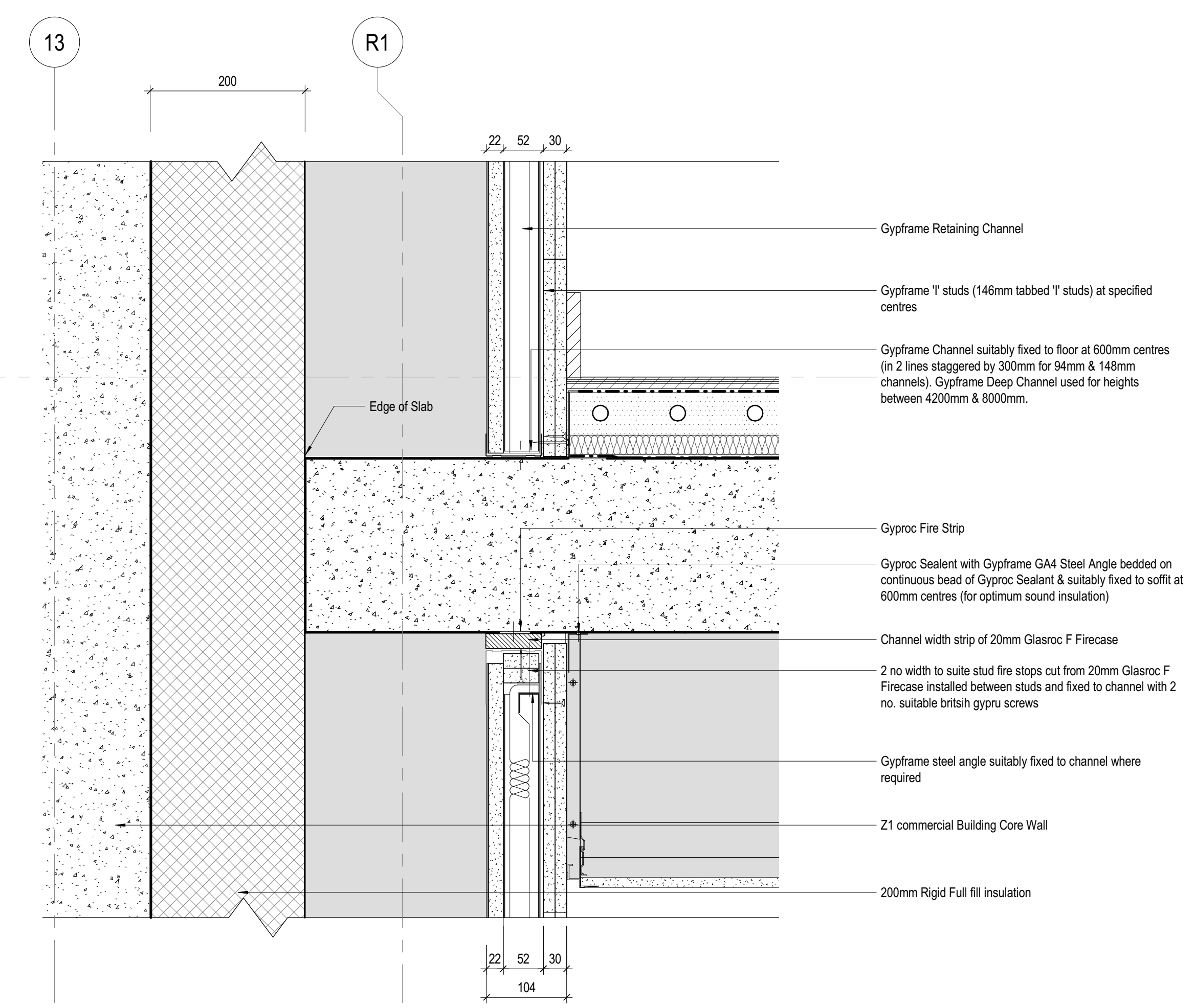
5 Enlarged Head and Base detail of shaft wall 1:5
