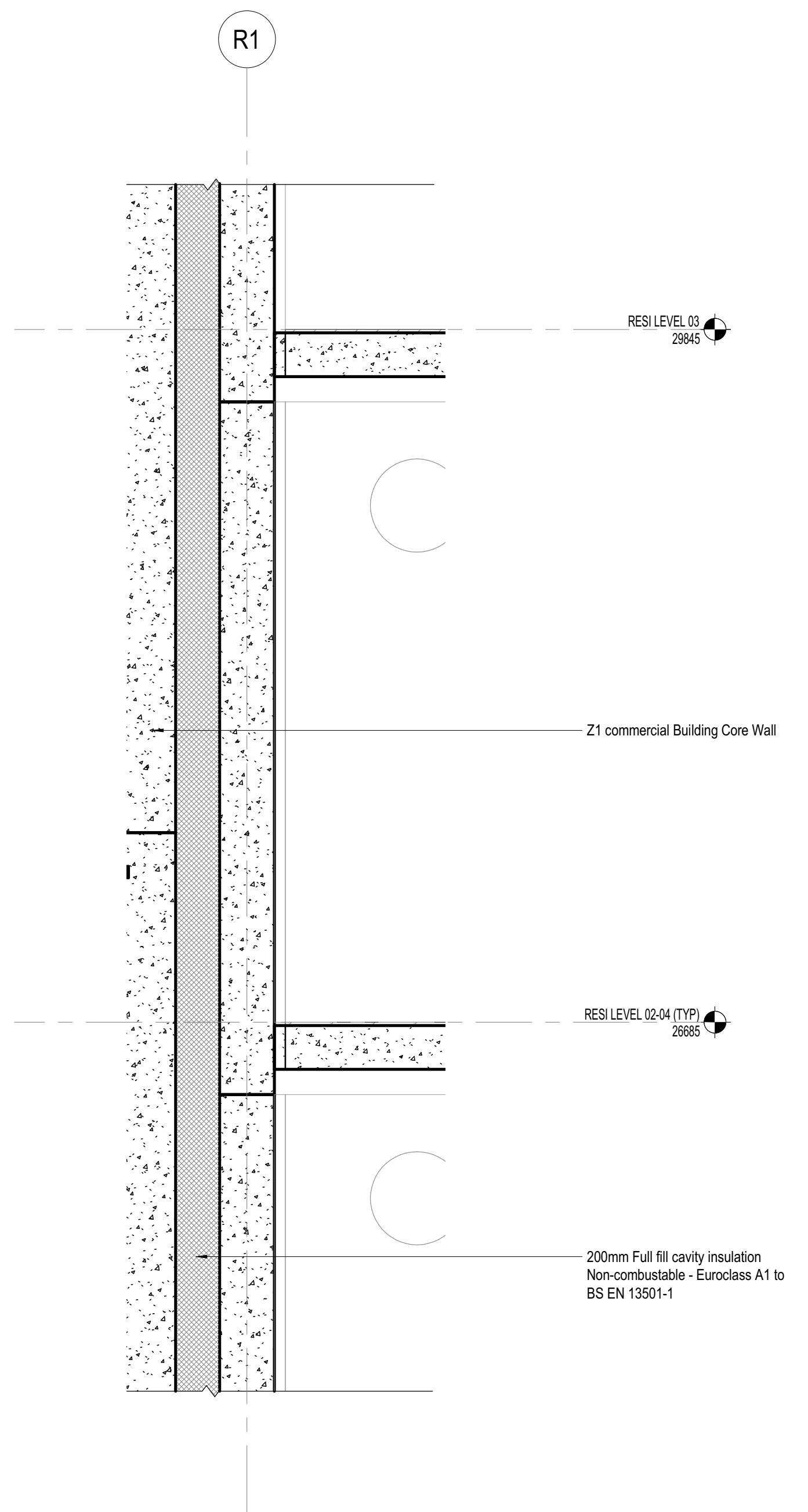
3 Typical section through concrete walls 1:20
