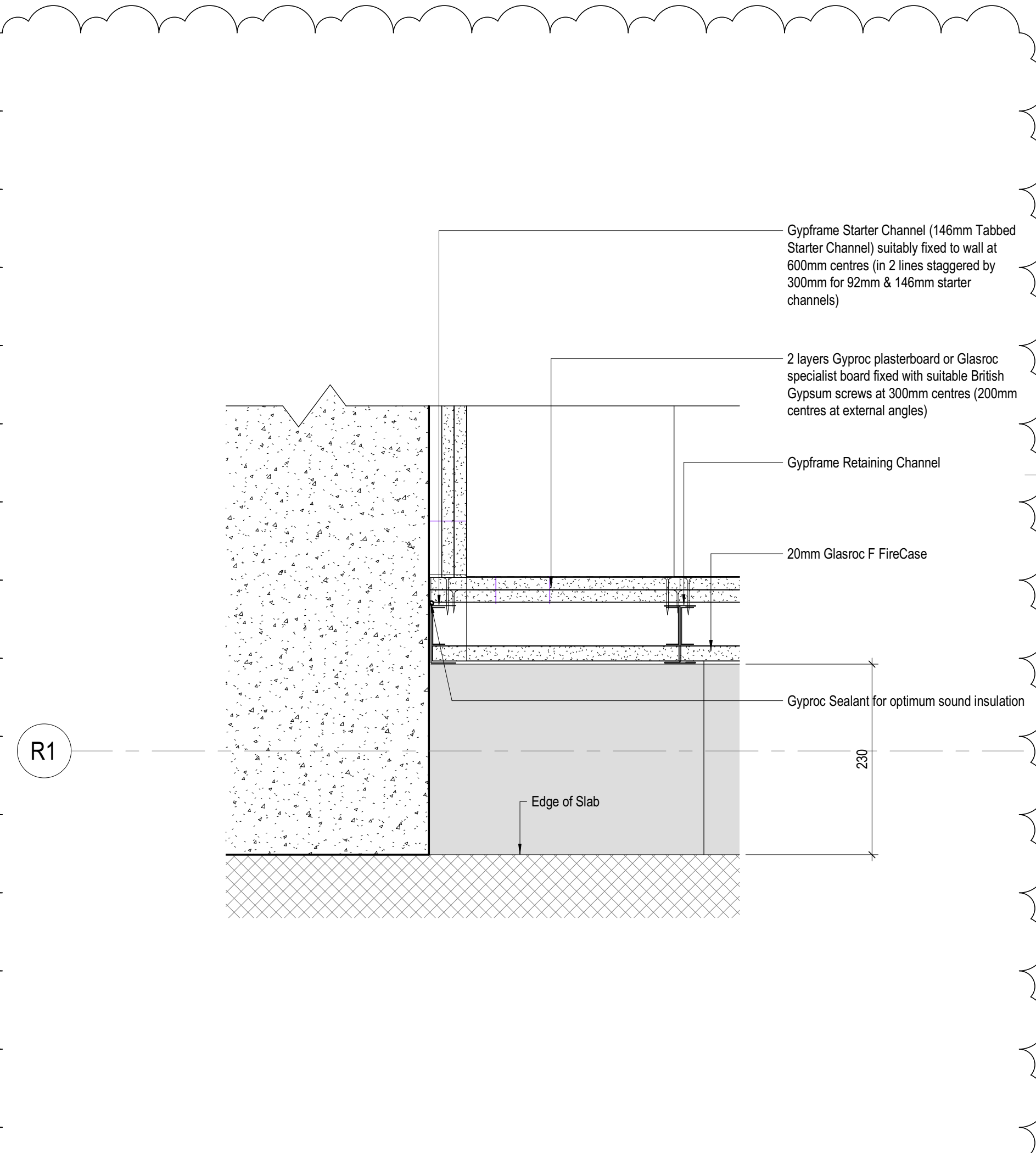
4 Typical Plan Abutment Detail 1:5 Detail applicable to wall abutment detail against column
