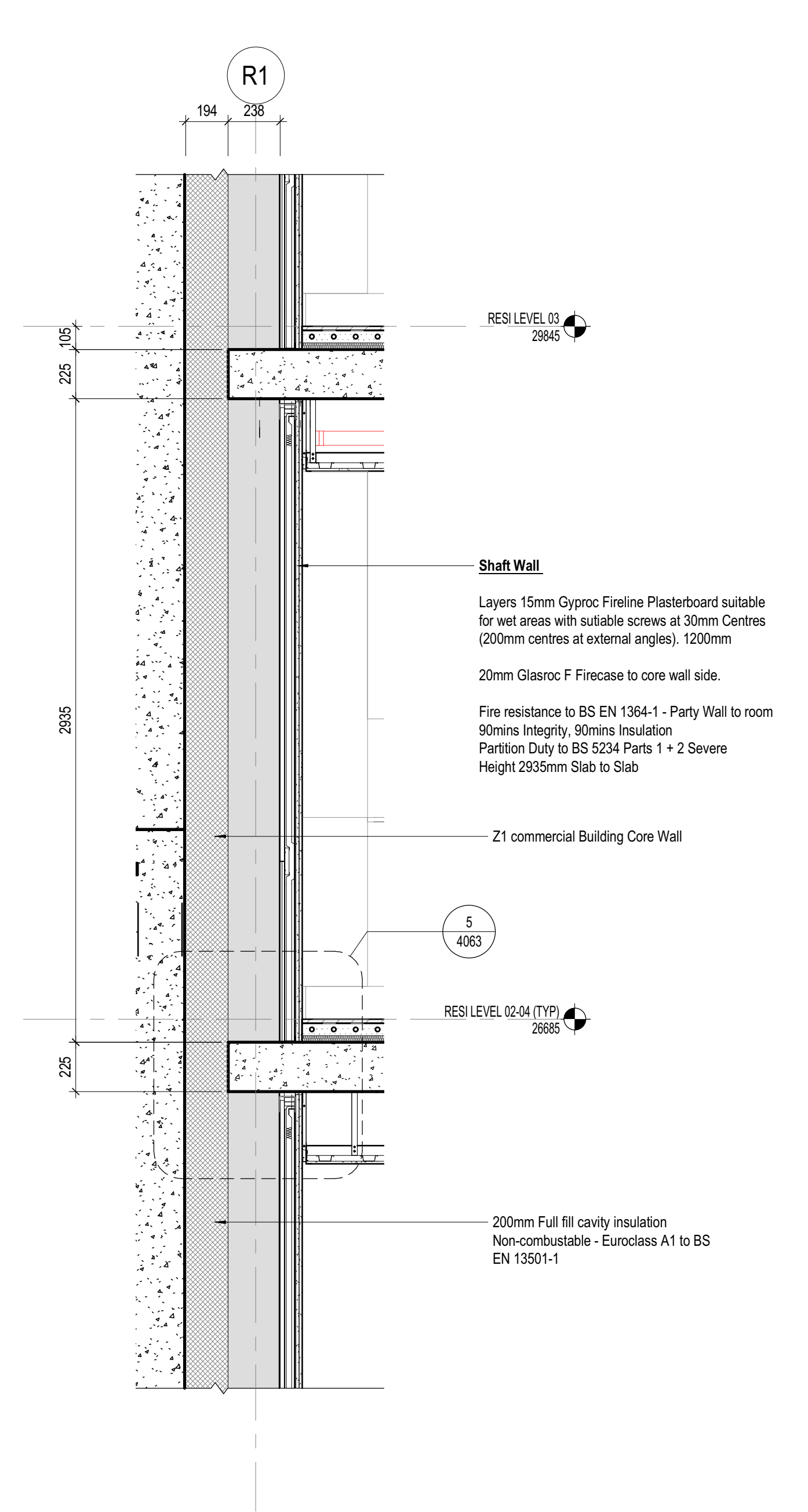
2 Typical Section through shaft wall 1:20
