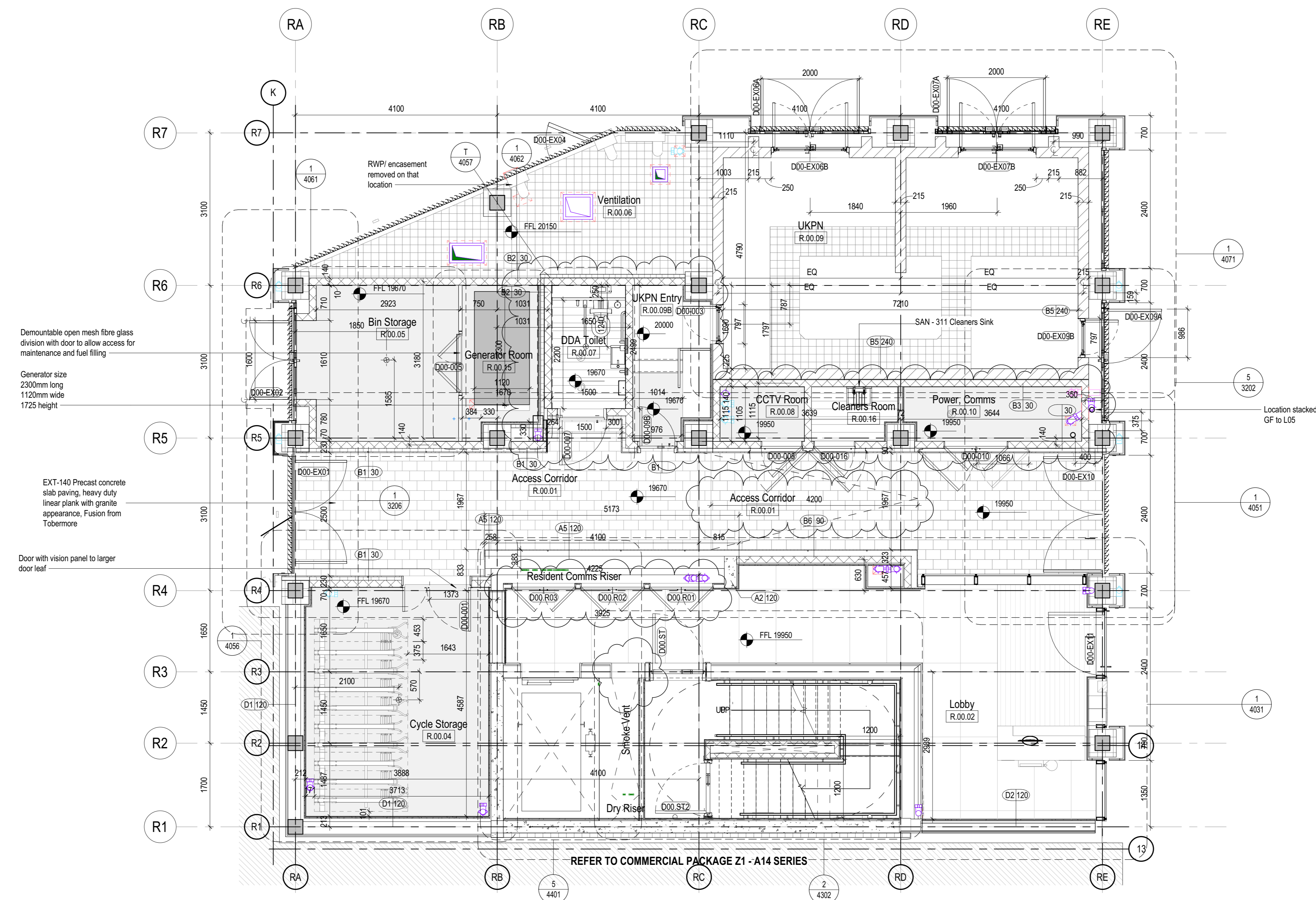
2 Consolidated Dimensions Plan Ground Level 1:50
