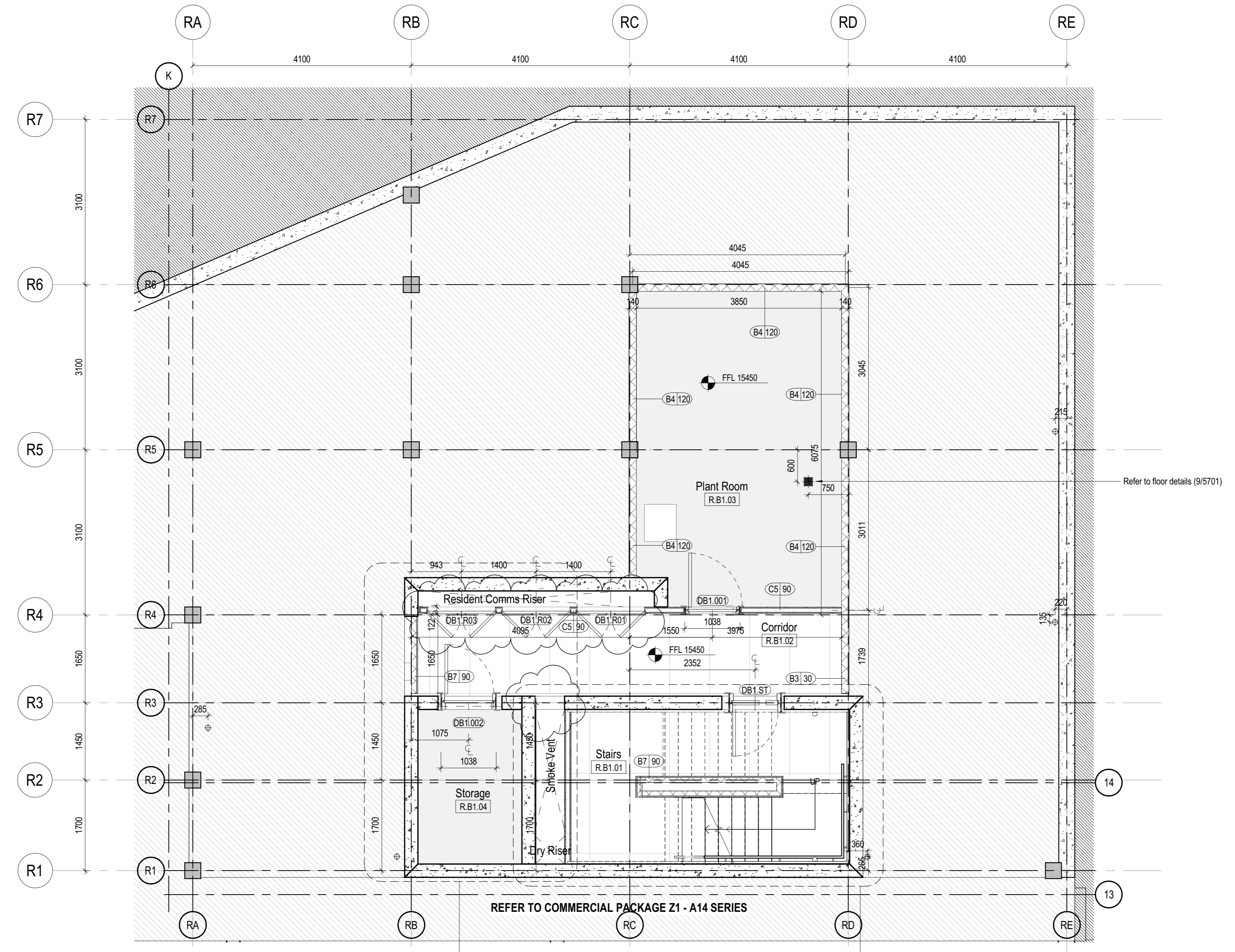
3 Consolidated Dimensions Plan Basement Level 1:50
