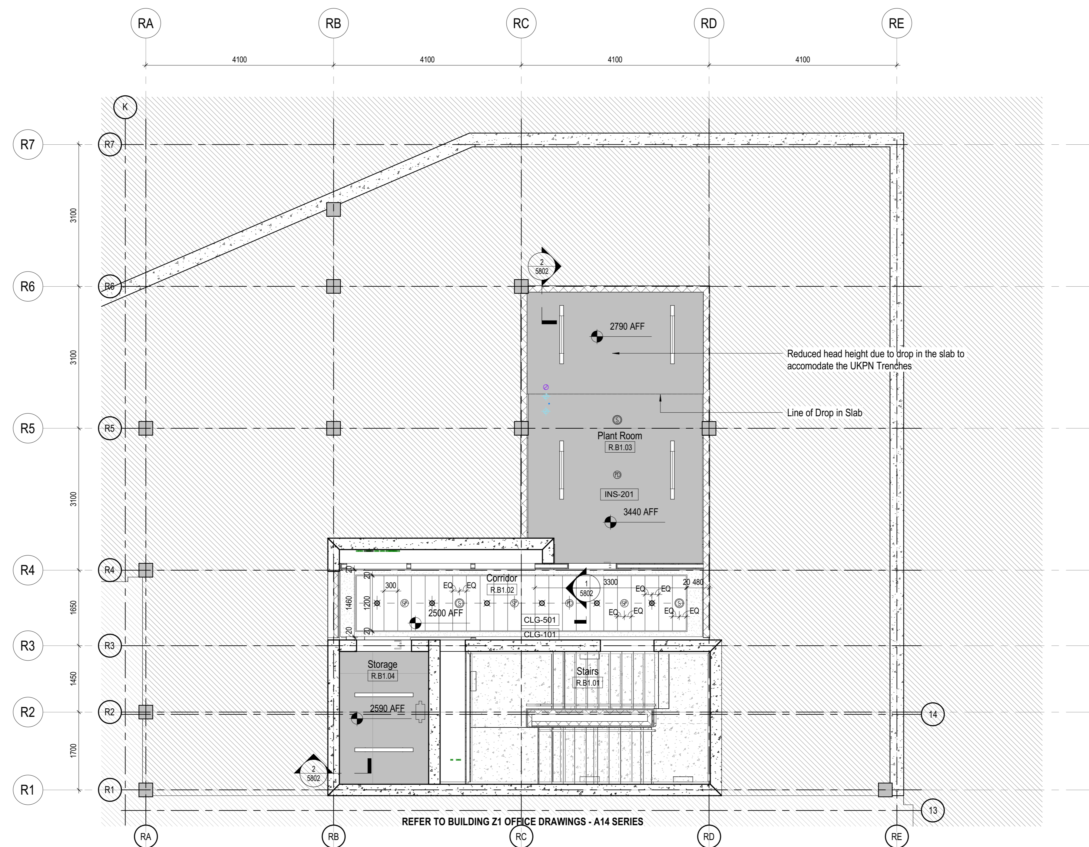
3 RCP BASEMENT LEVEL 1:50 REFER TO THE RELEVANT A40-ENLARGED PLANS DRAWINGS AND A58 SERIES FOR RCP DETAILS Those drawings are for setting out purposes only, refer to MEP contractual documents for specs and services layouts.
