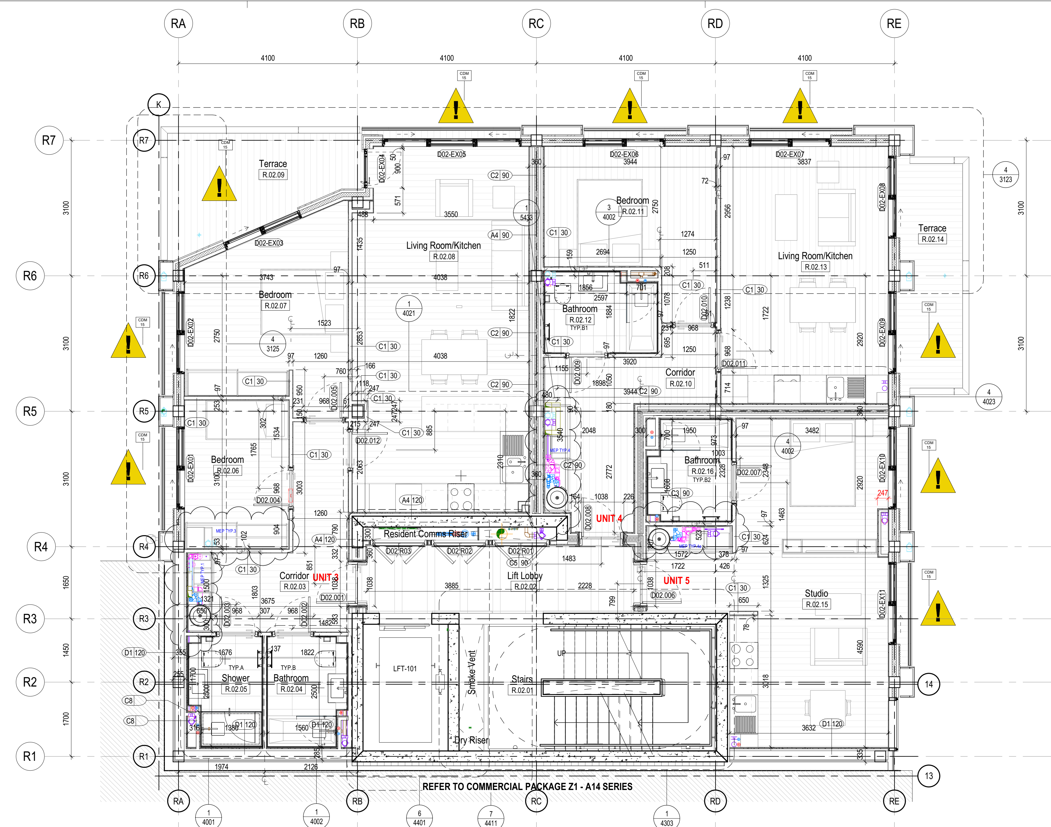
2 Consolidated Dimensions Plan Level 02 1 : 50 Bathroom Layouts noted on this plan should be viewed along with A40 Series Enlarged Plans - Bathrooms
