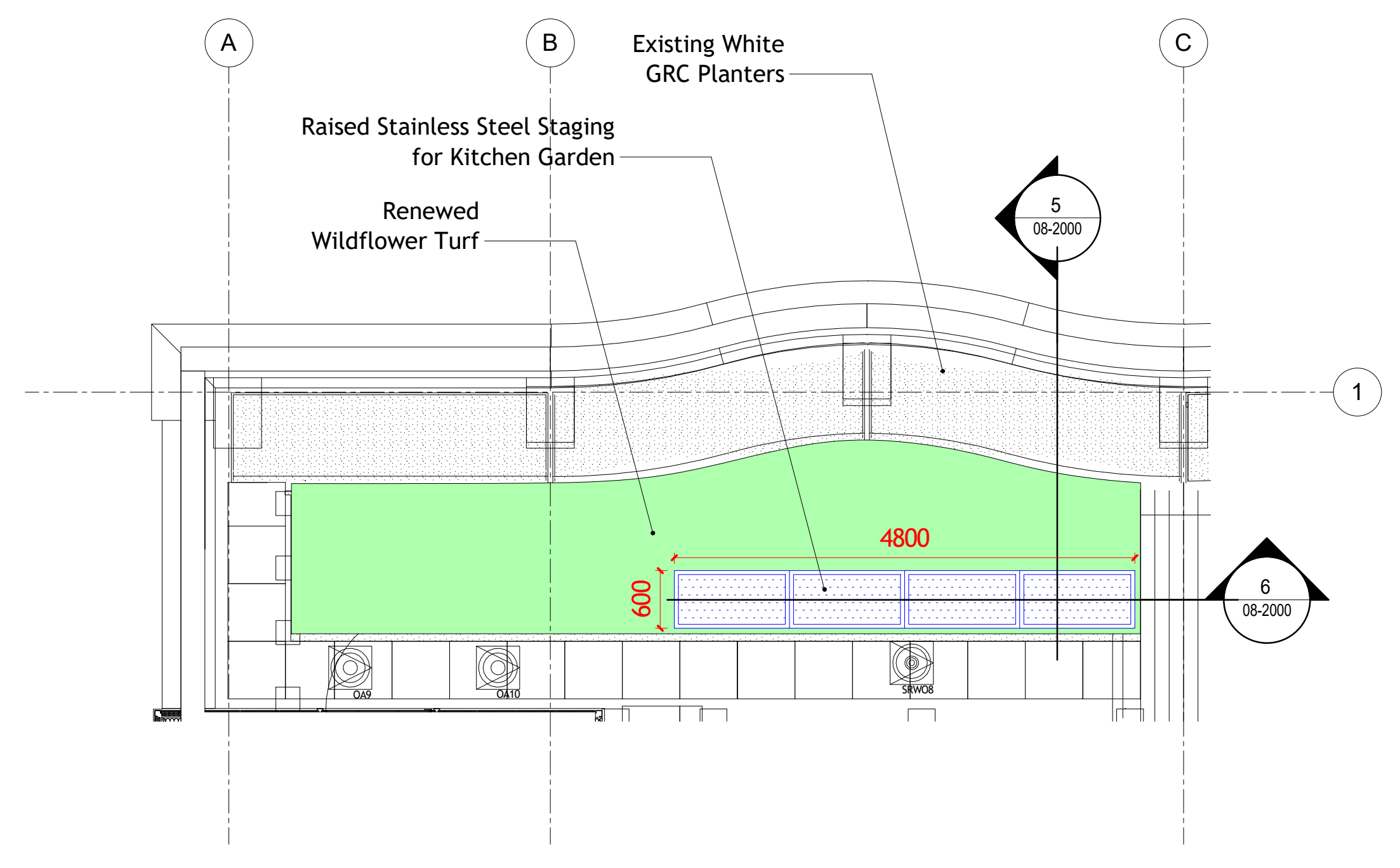
1 Proposed Level 05 Roof Terrace -West Detail 1 : 50
