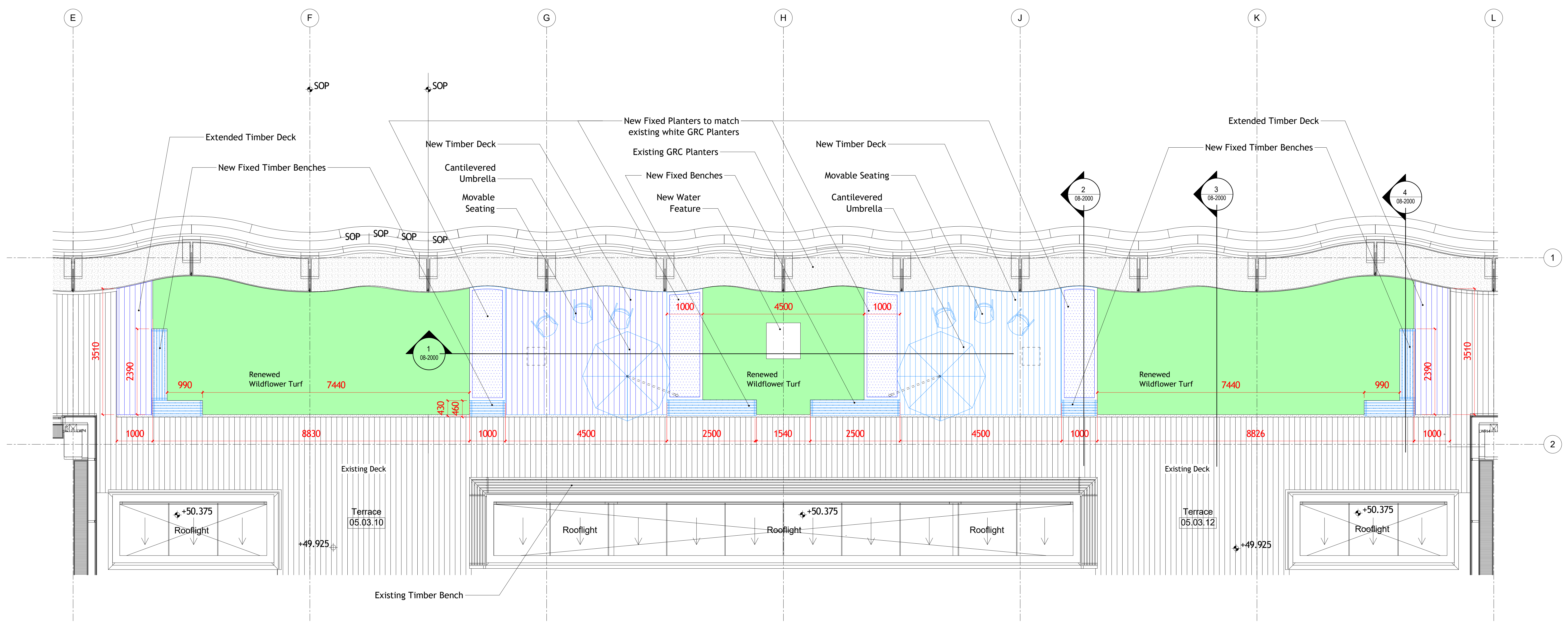
2 Proposed Level 05 Roof Terrace - Central Detail 1 : 50
