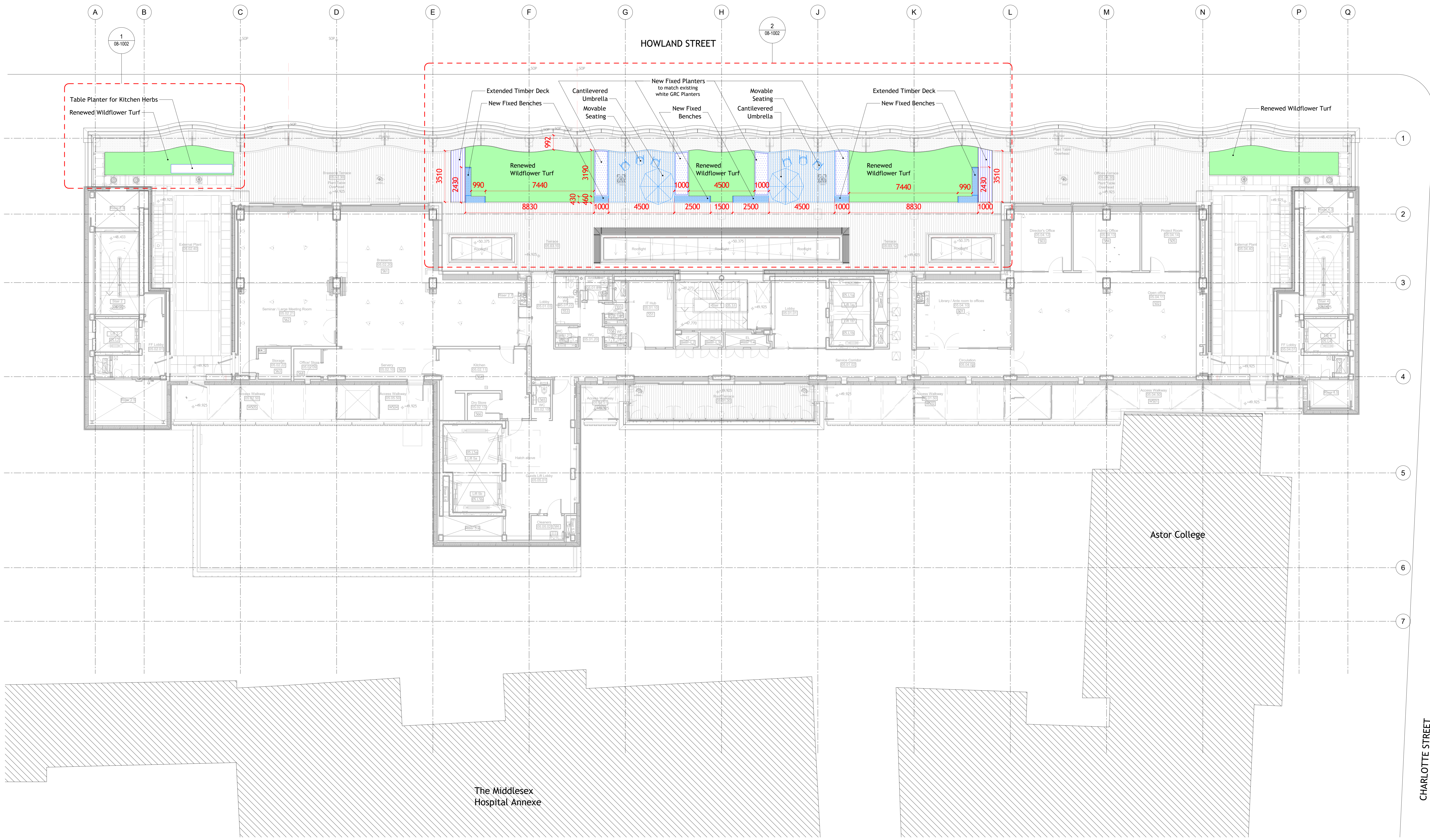
1 Proposed Level 05 Roof Terrace 1 : 100
