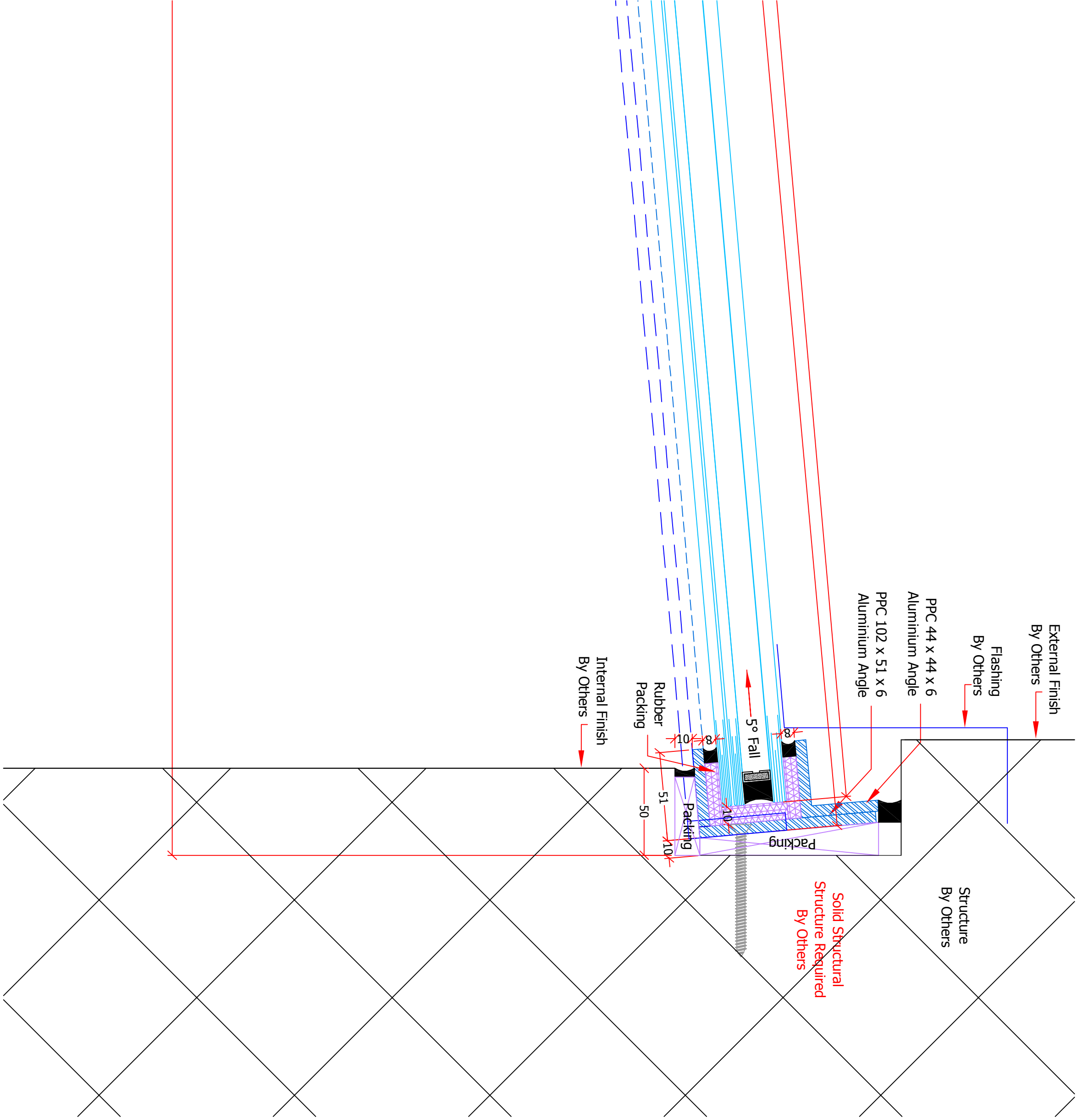
RL01 - Section Detail B:B SCALE 1:2
