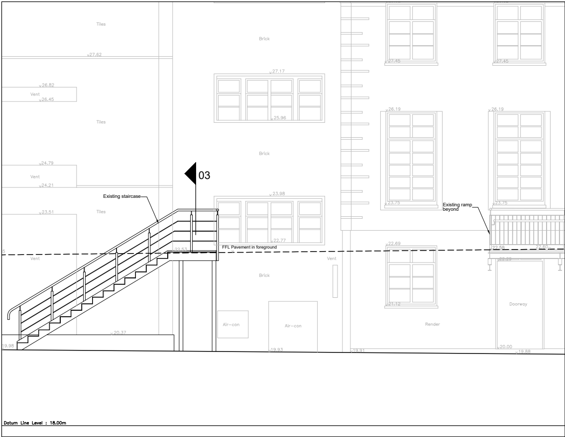
02 Existing Elevation Through Well (02)001 1:100 @ A3
