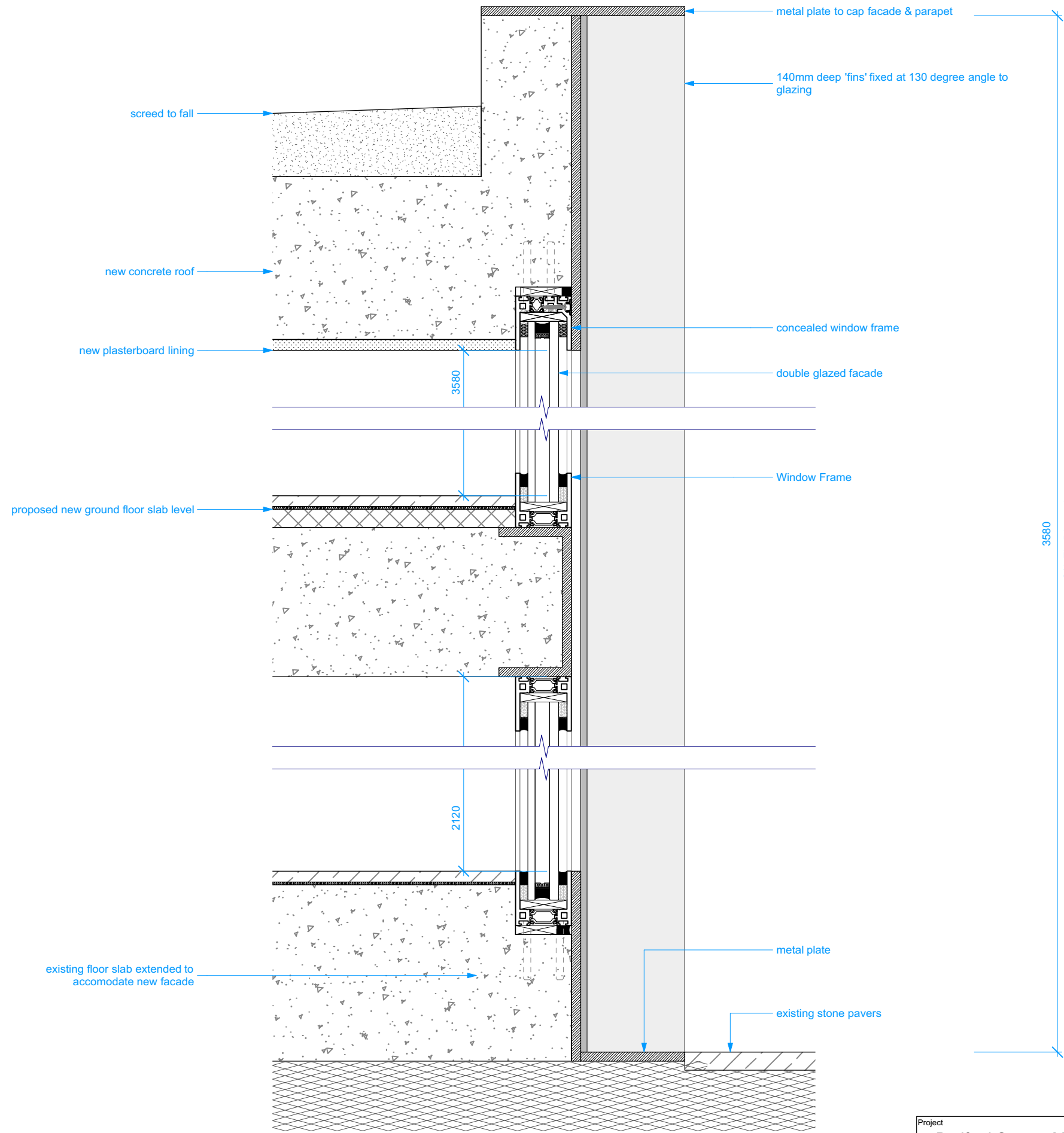
Proposed Section BB - Detail A Scale: 1:5 @ A3
