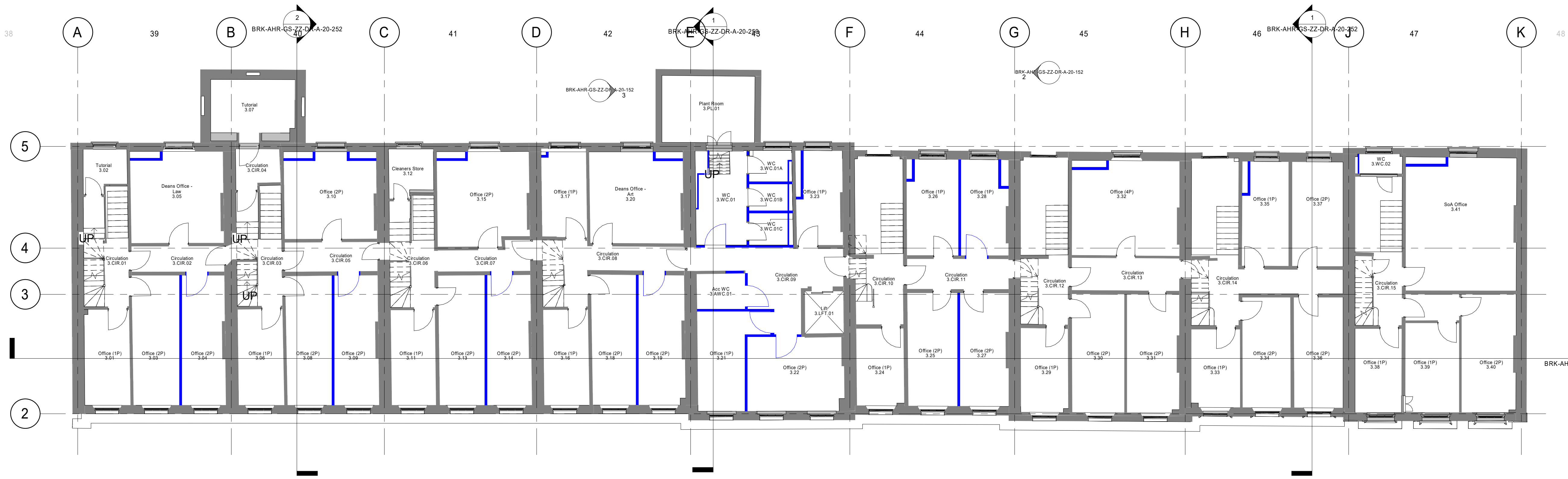
1. Planning - LEVEL 03 - Proposed 1 : 100
