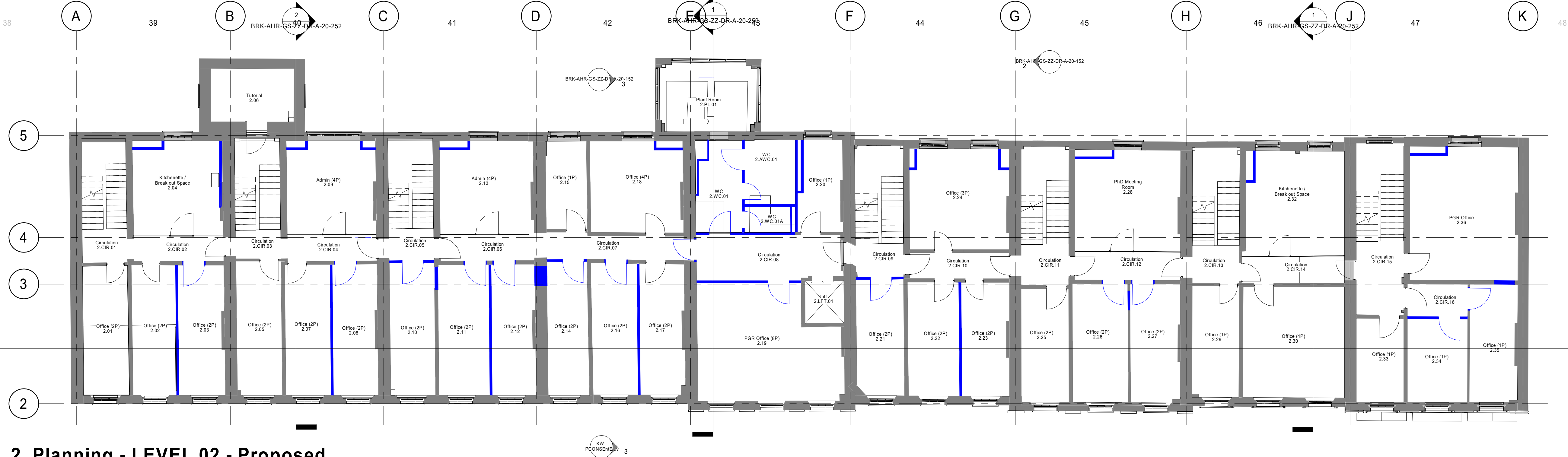
2. Planning - LEVEL 02 - Proposed 1 : 100
