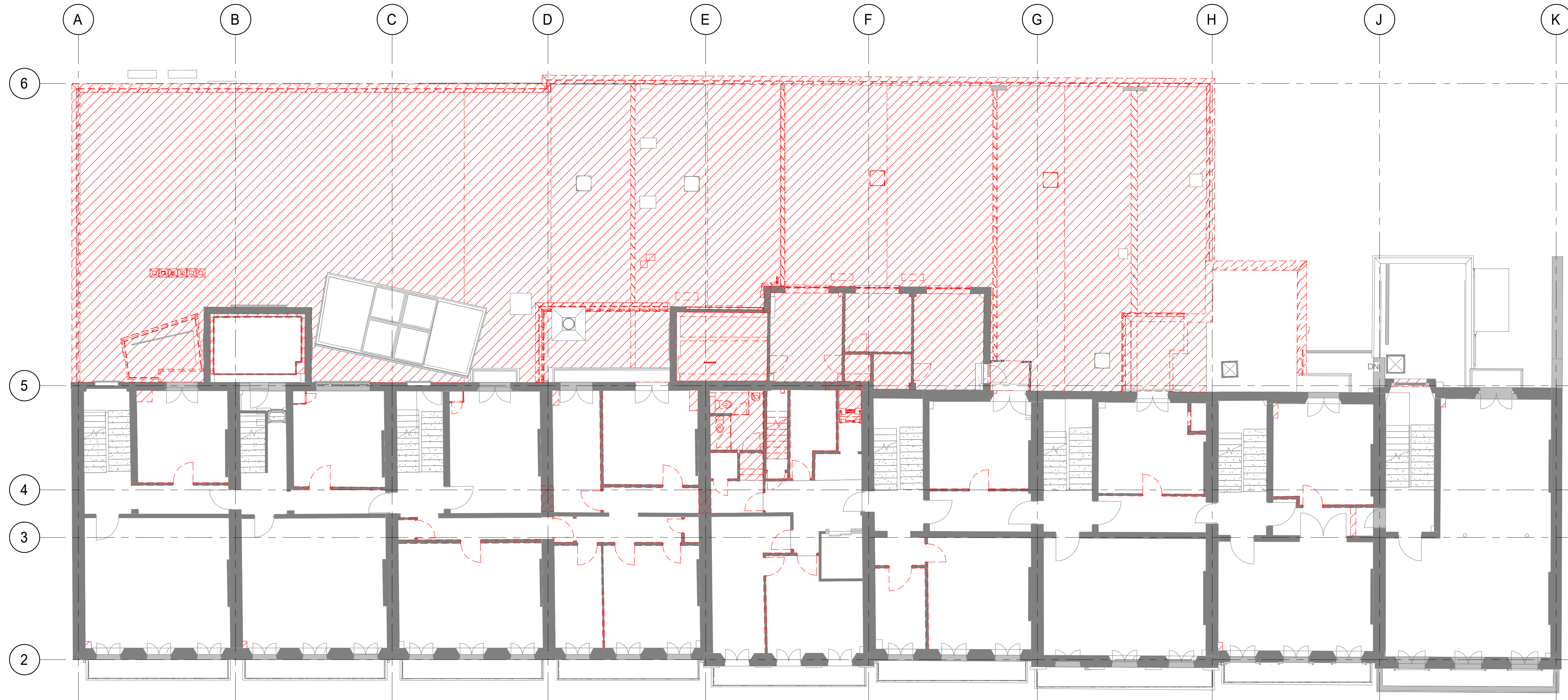
1. Planning - LEVEL 01 - Demolition Plan 1 : 100
