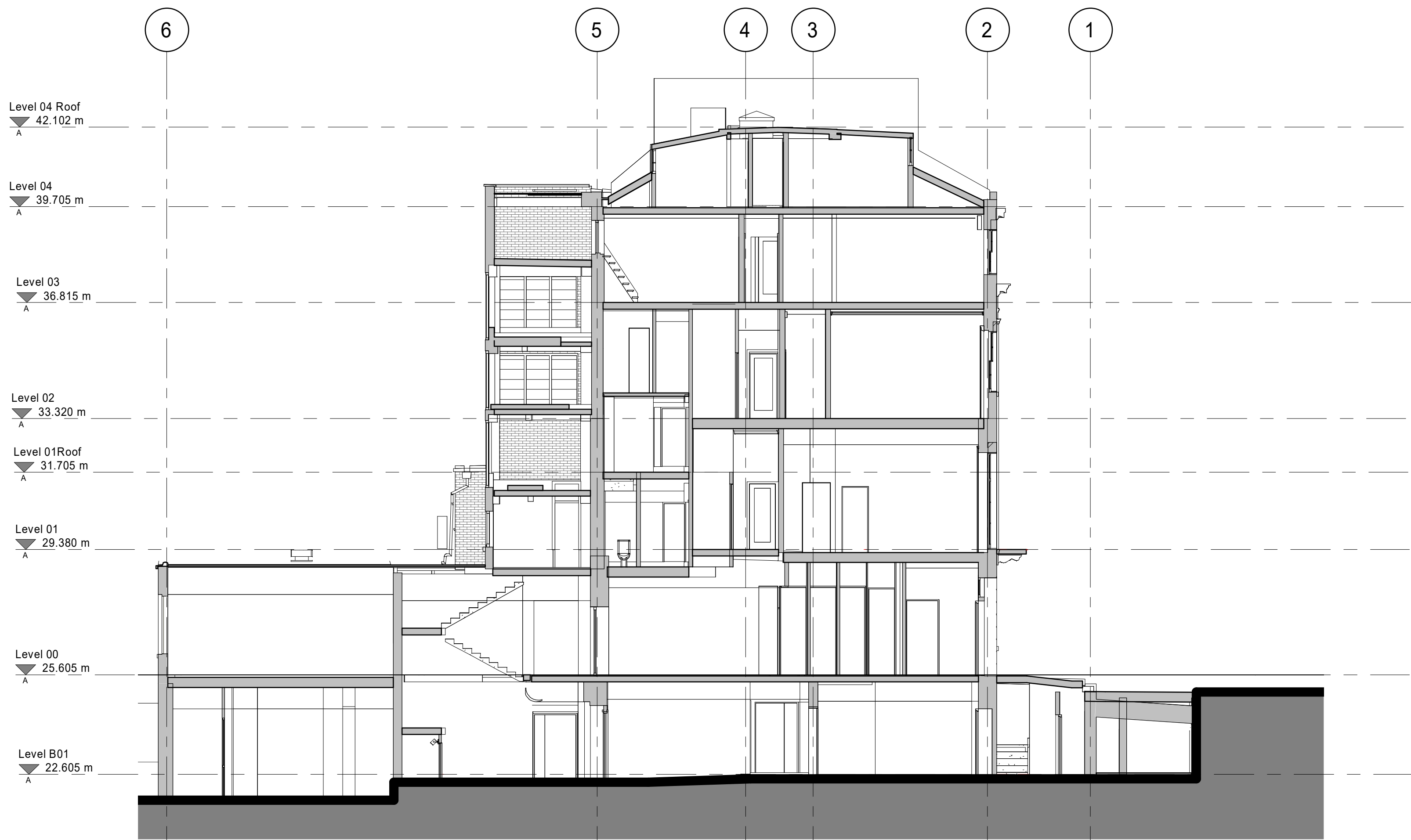
2. Planning - Existing Section - Section 01 1 : 100
