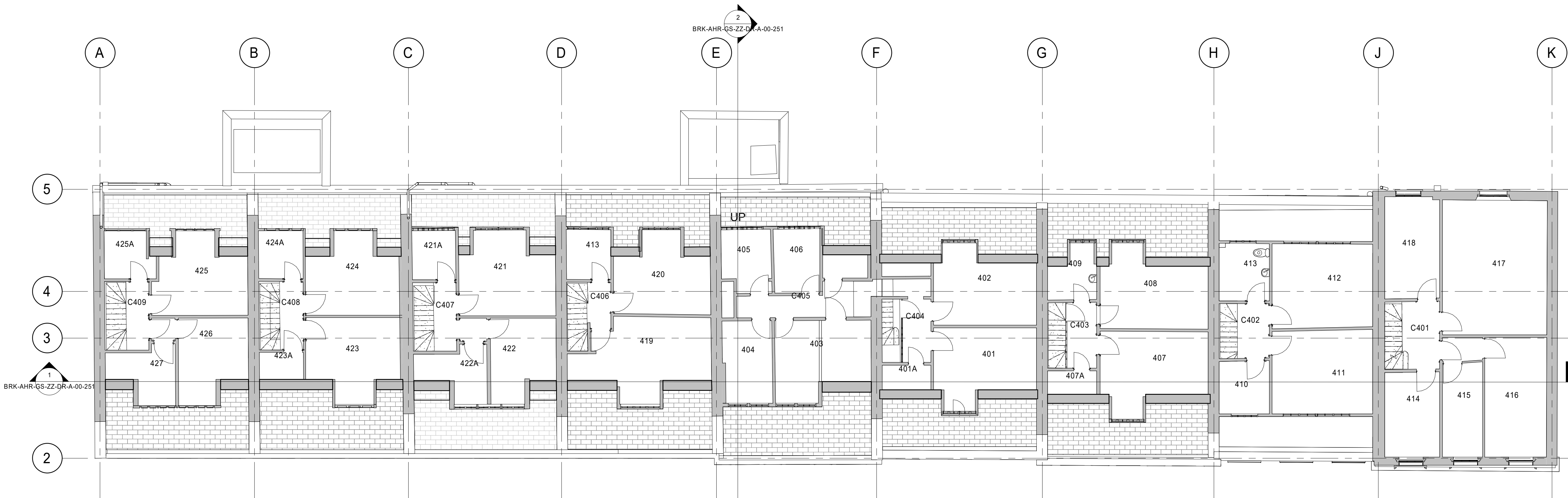
2. Planning - LEVEL 04 - Existing 1 : 100
