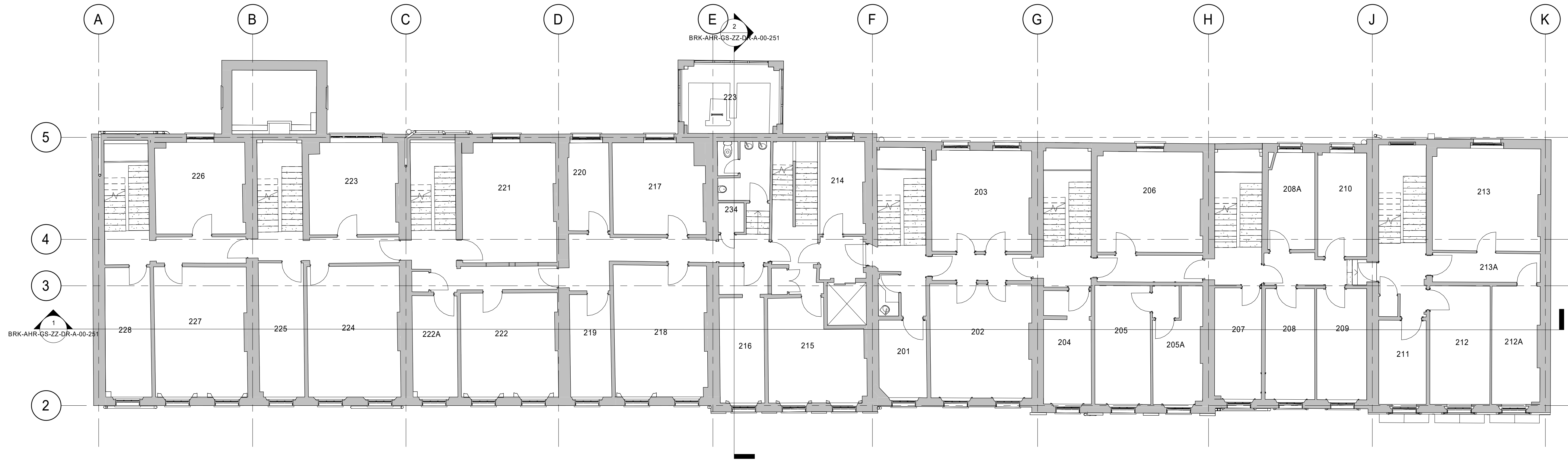
2. Planning - LEVEL 02 - Existing 1 : 100
