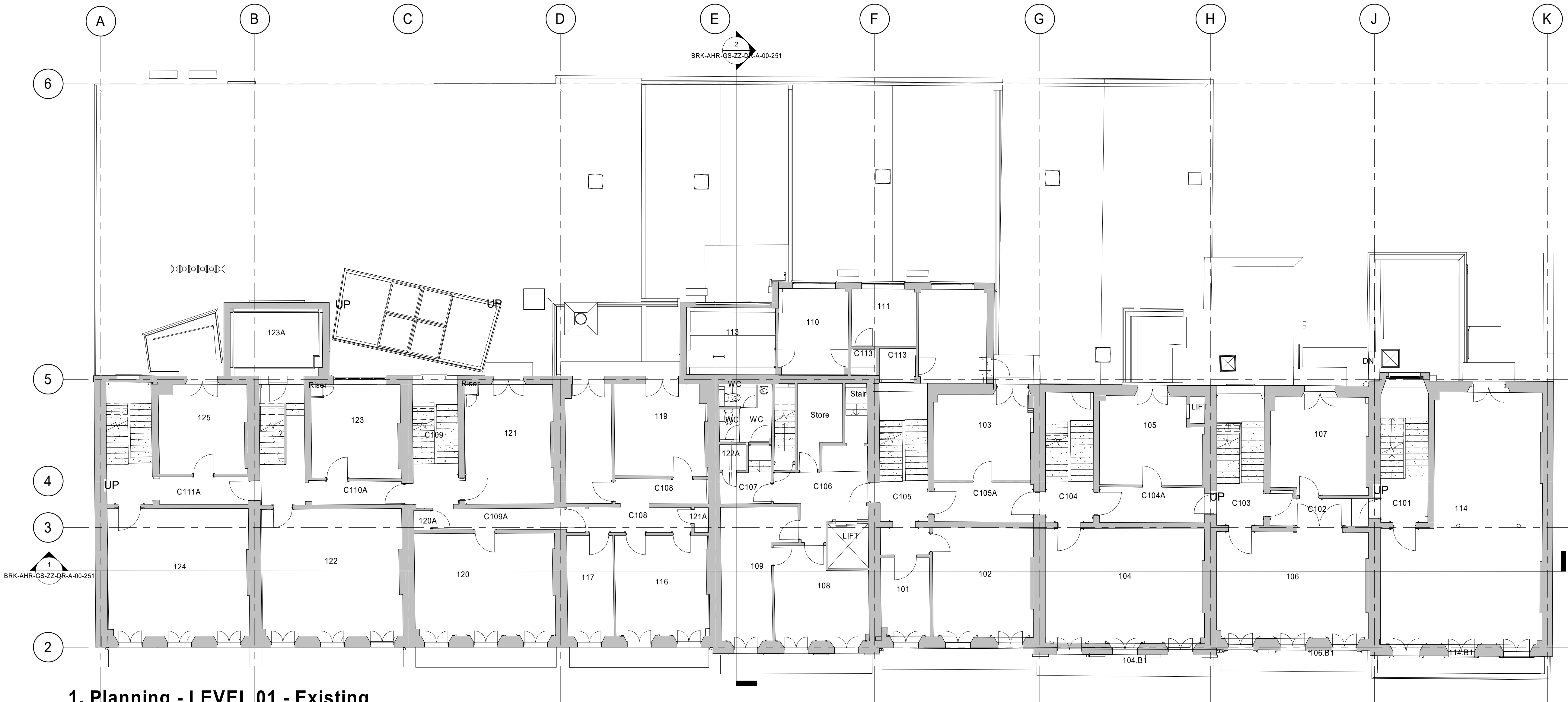
1. Planning - LEVEL 01 - Existing 1 : 100
