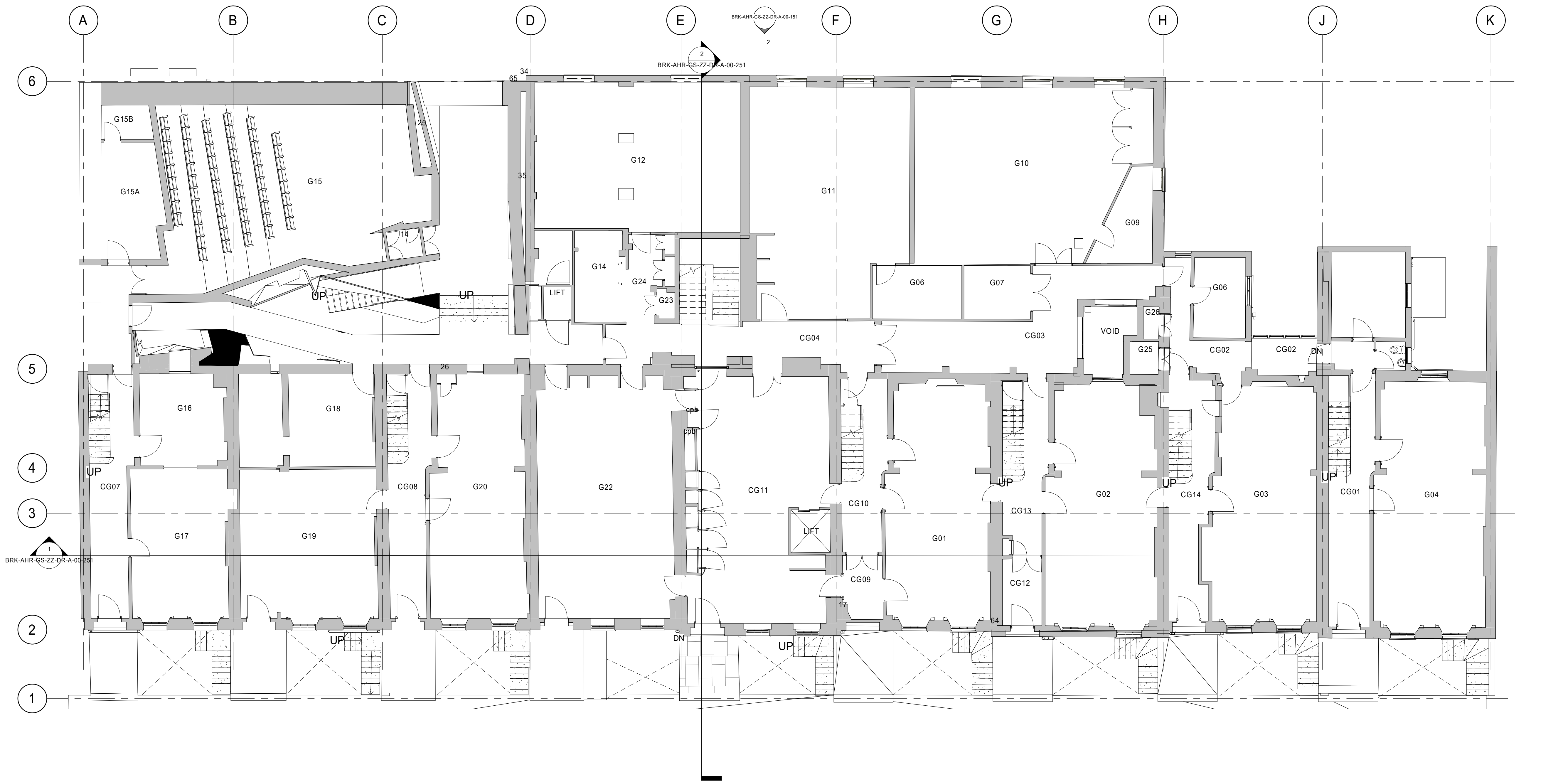
1. Planning - LEVEL 00 - Existing 1 : 100
