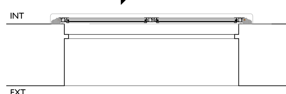
WINDOW TYPE WT 021
